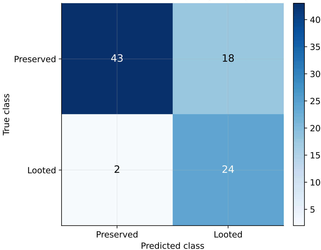
Test confusion matrix (counts)
