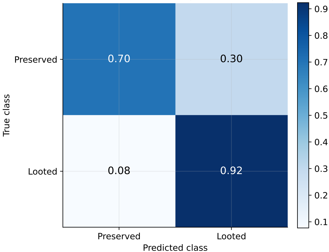
Test confusion matrix (row-normalized)
