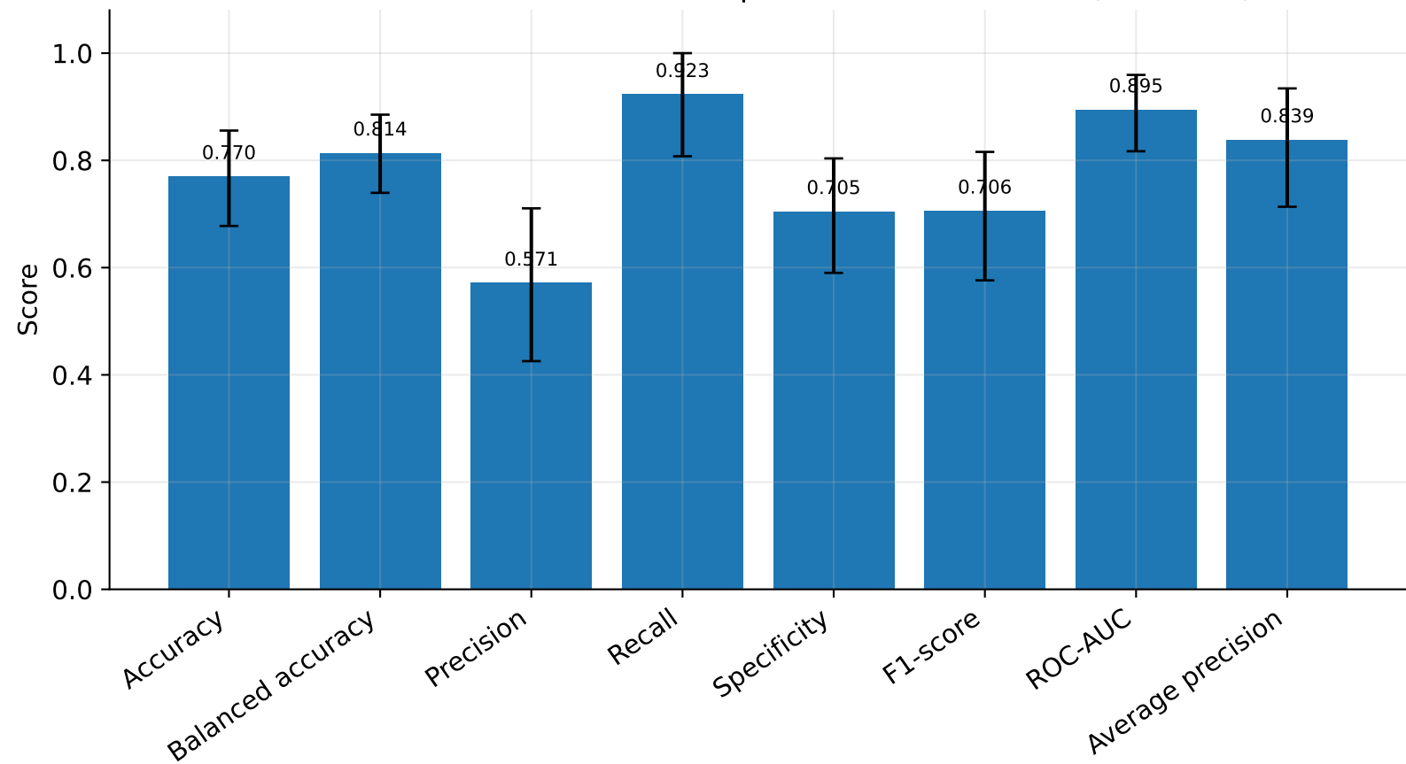
Test metrics with 95% bootstrap confidence intervals (site-level)
