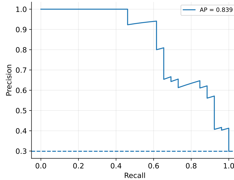
Precision-recall curve
