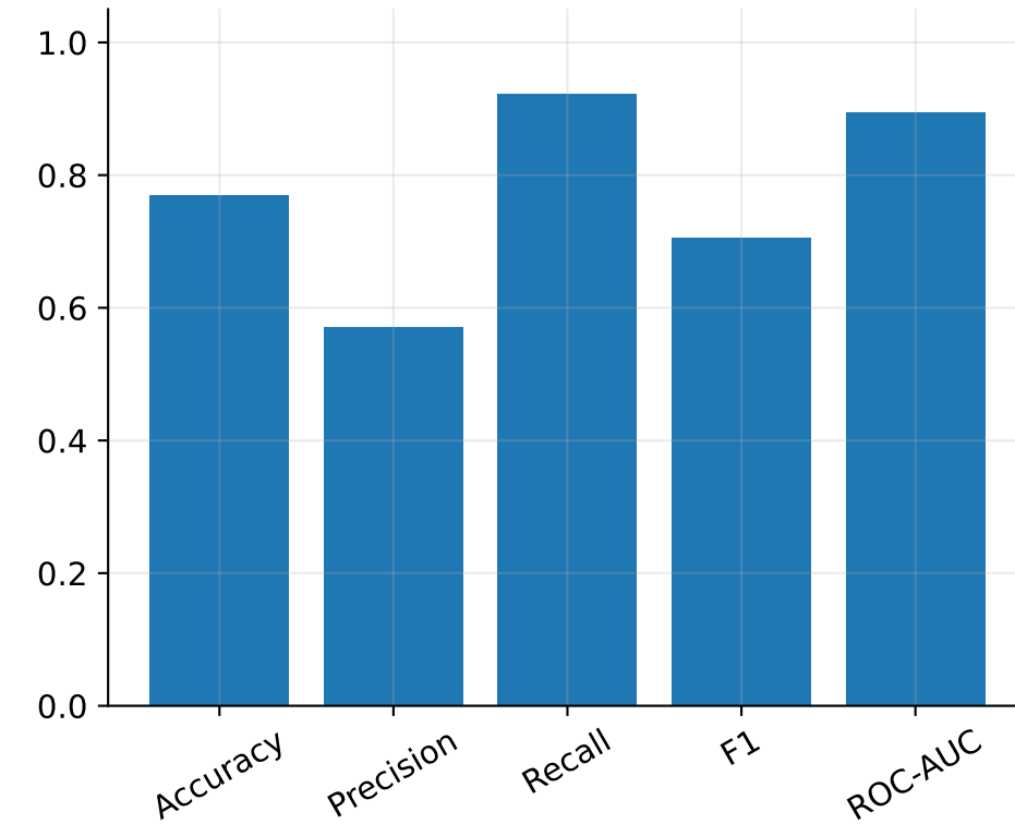
Test metrics
