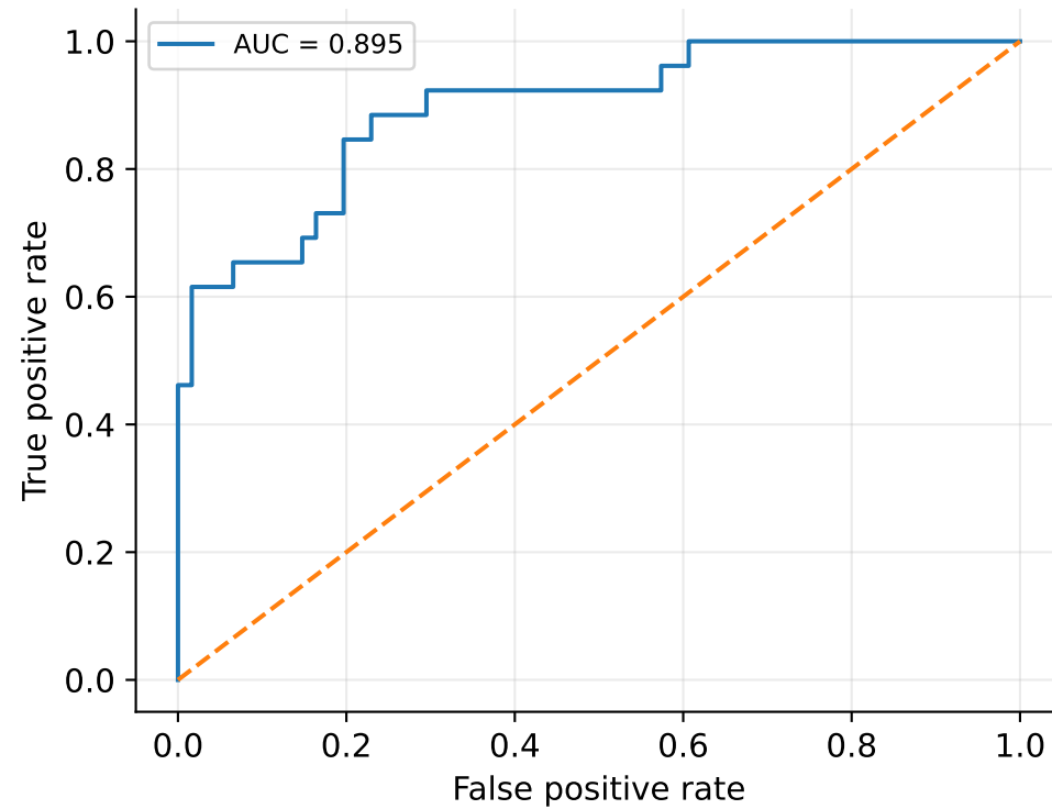
ROC curve
