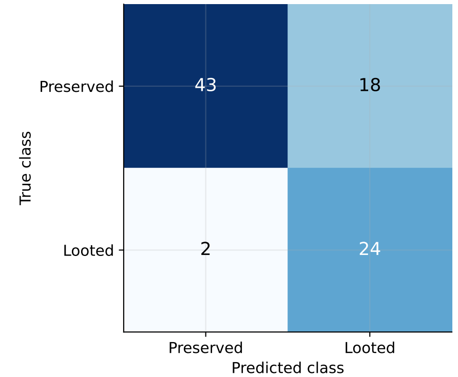
Test metrics
