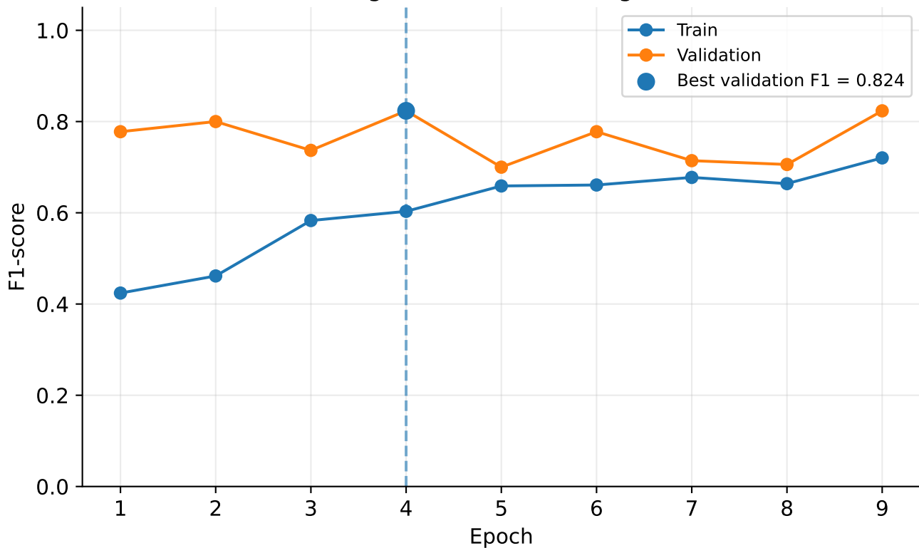
Two-frame change ResNet18 learning curve: F1-score
