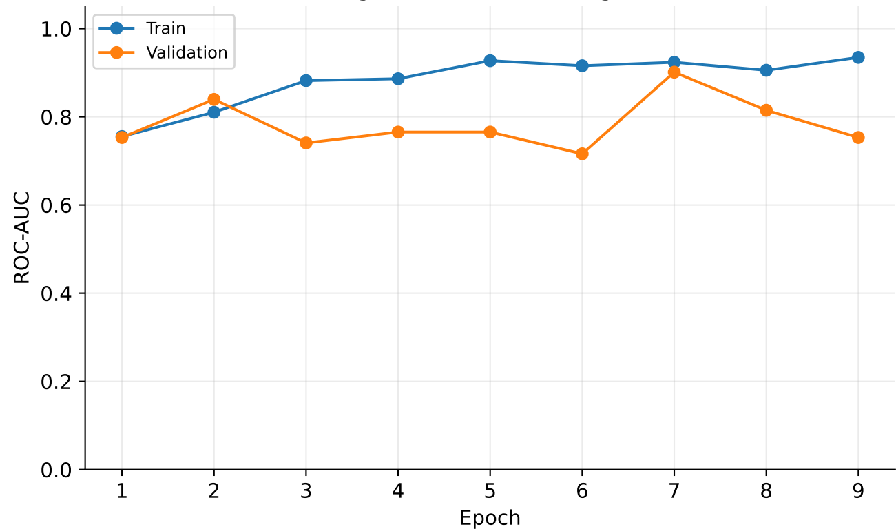
Two-frame change ResNet18 learning curve: ROC-AUC
