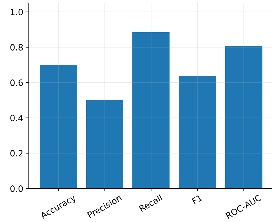
Test metrics
