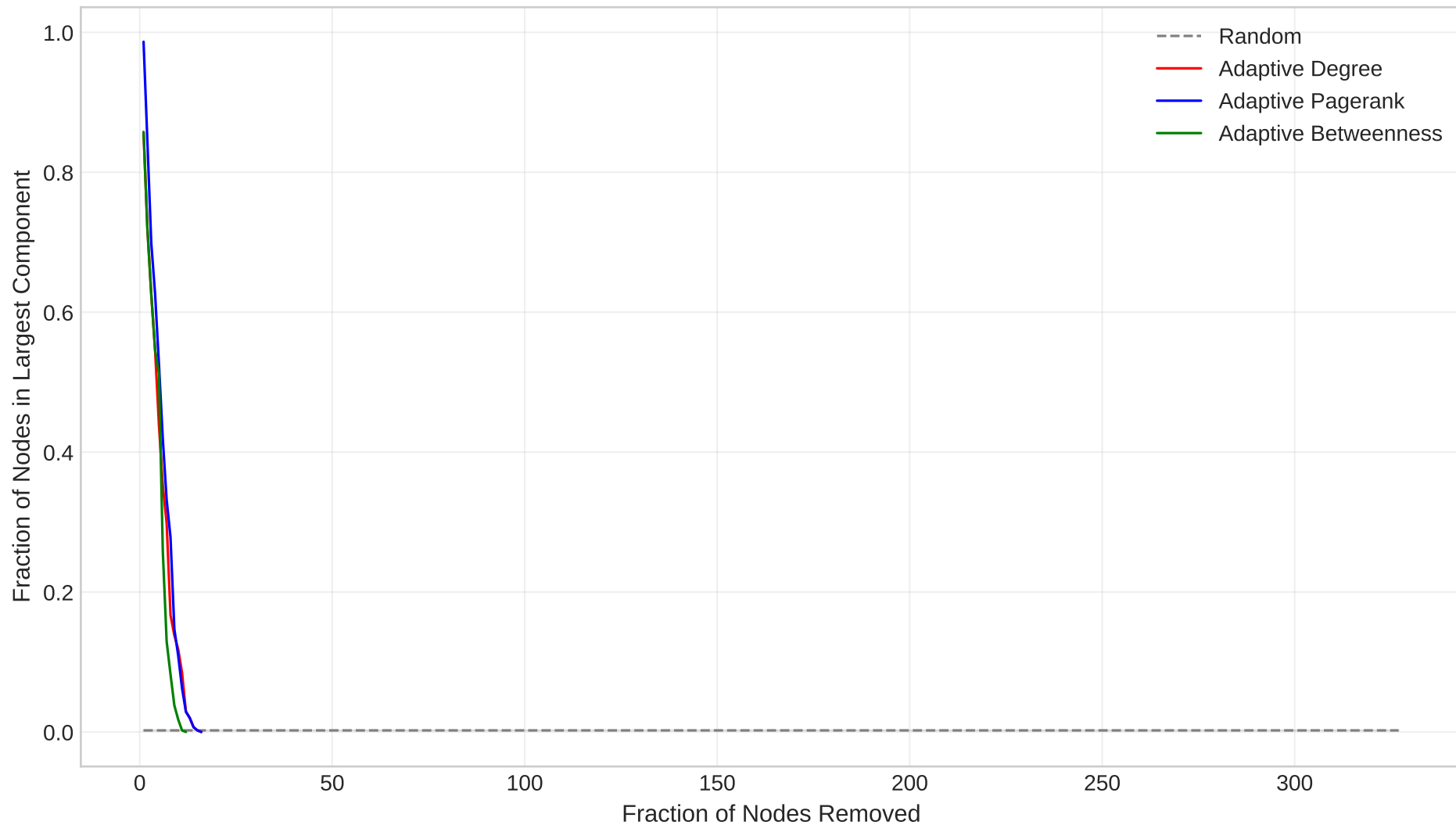
Robustness Curves: Random vs Targeted Attacks
