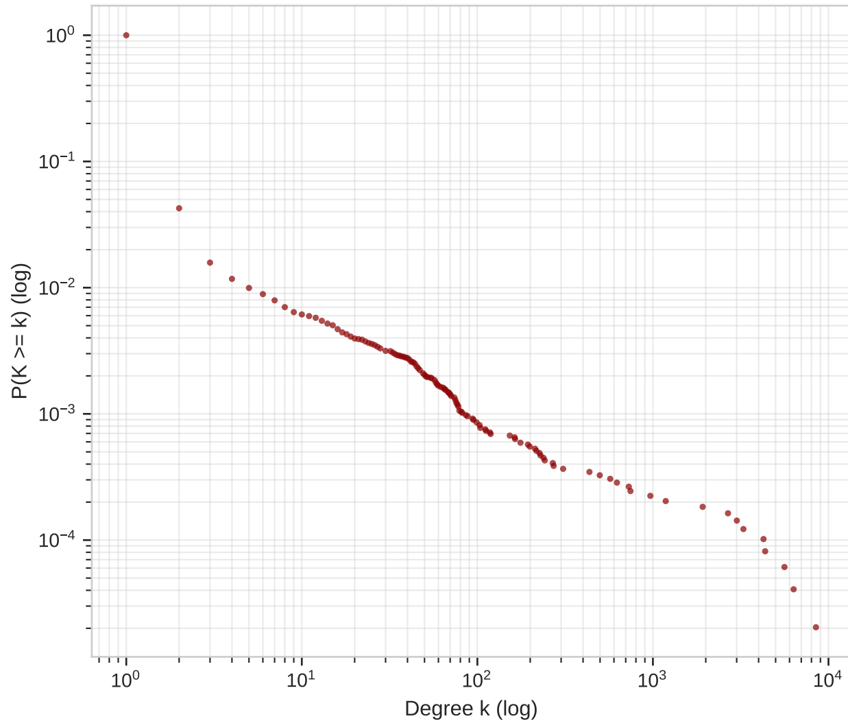
Degree Distribution (CCDF)
