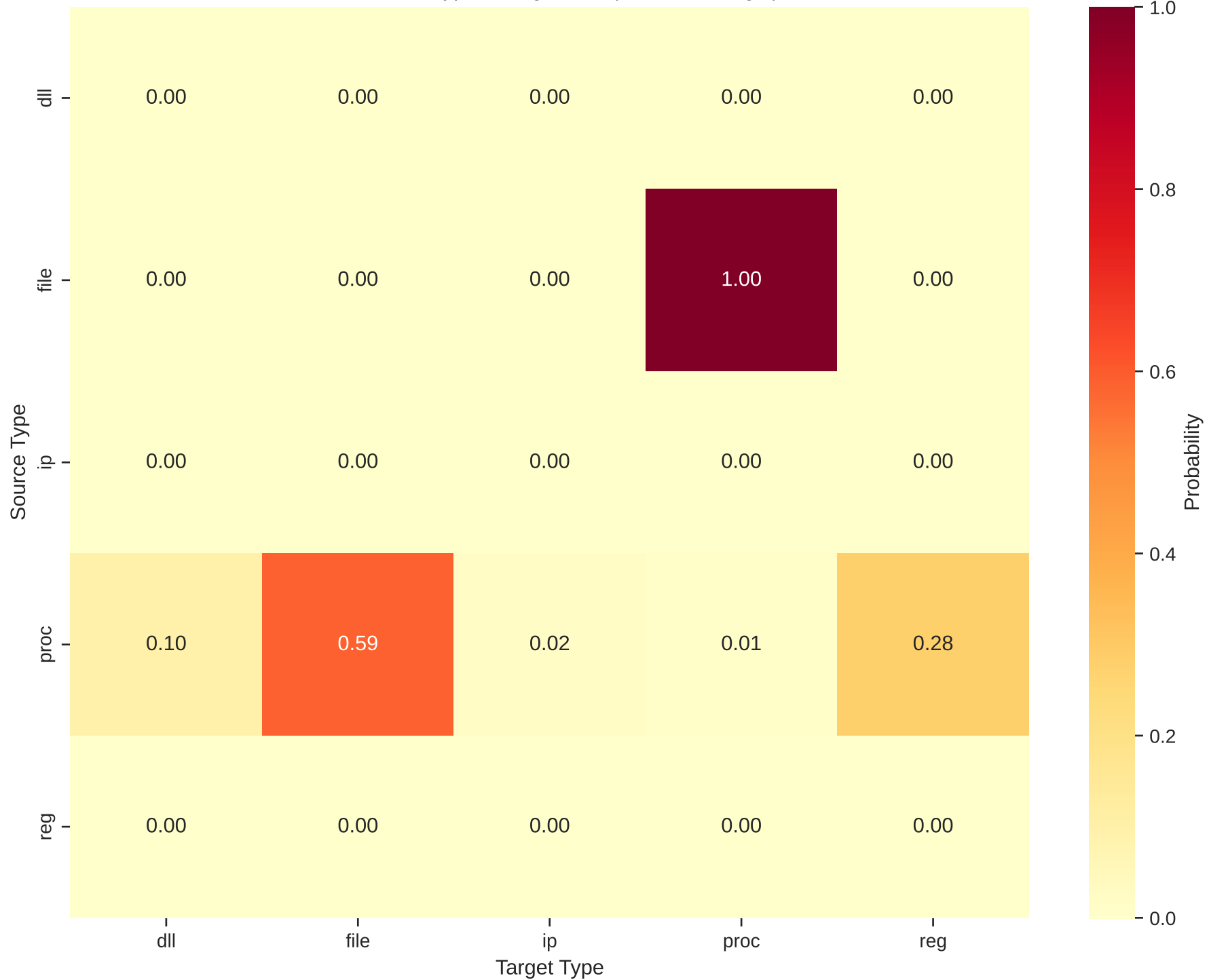
Normalized Type Mixing Matrix (Source -> Target)
