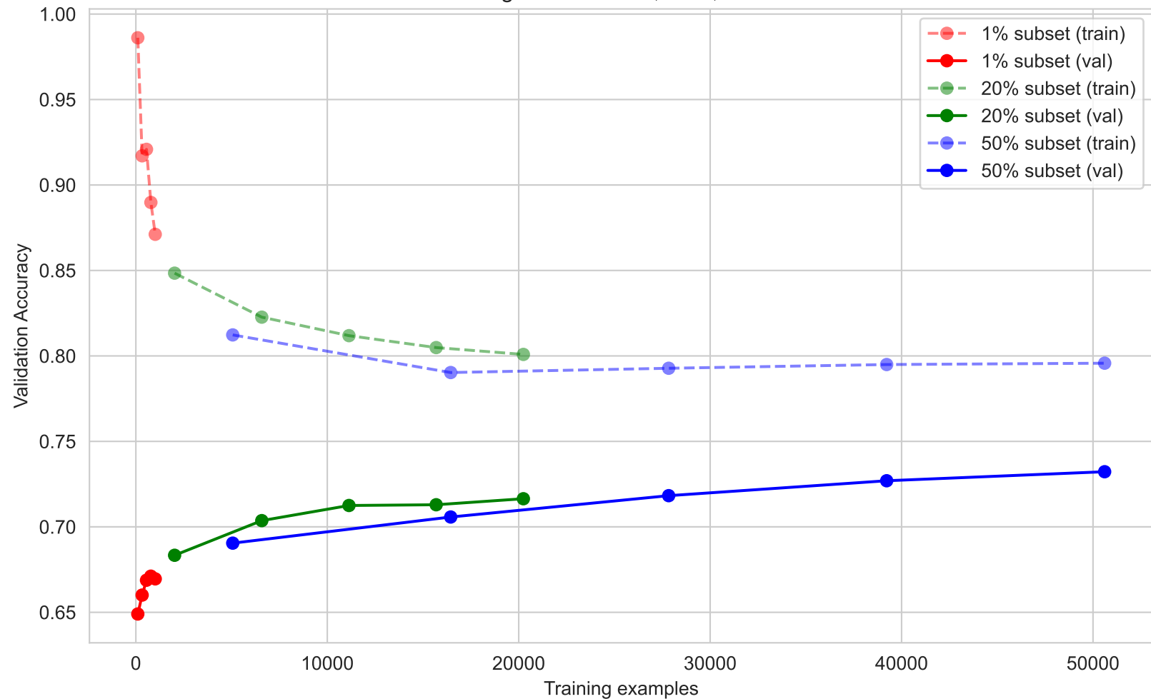
NB Learning Curve for 1%, 20%, 50% subsets
