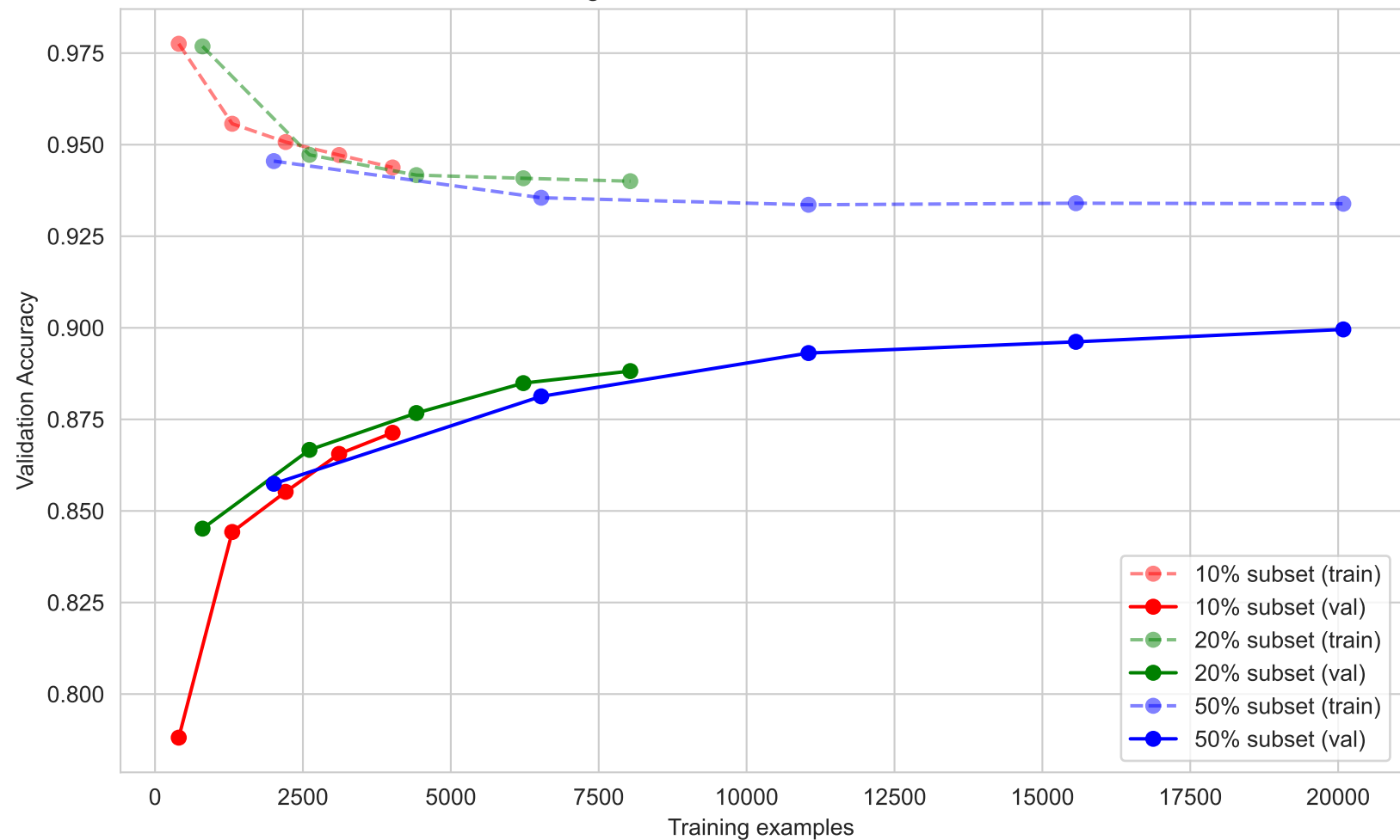
Learning Curve for 10%, 20%, 50% subsets
