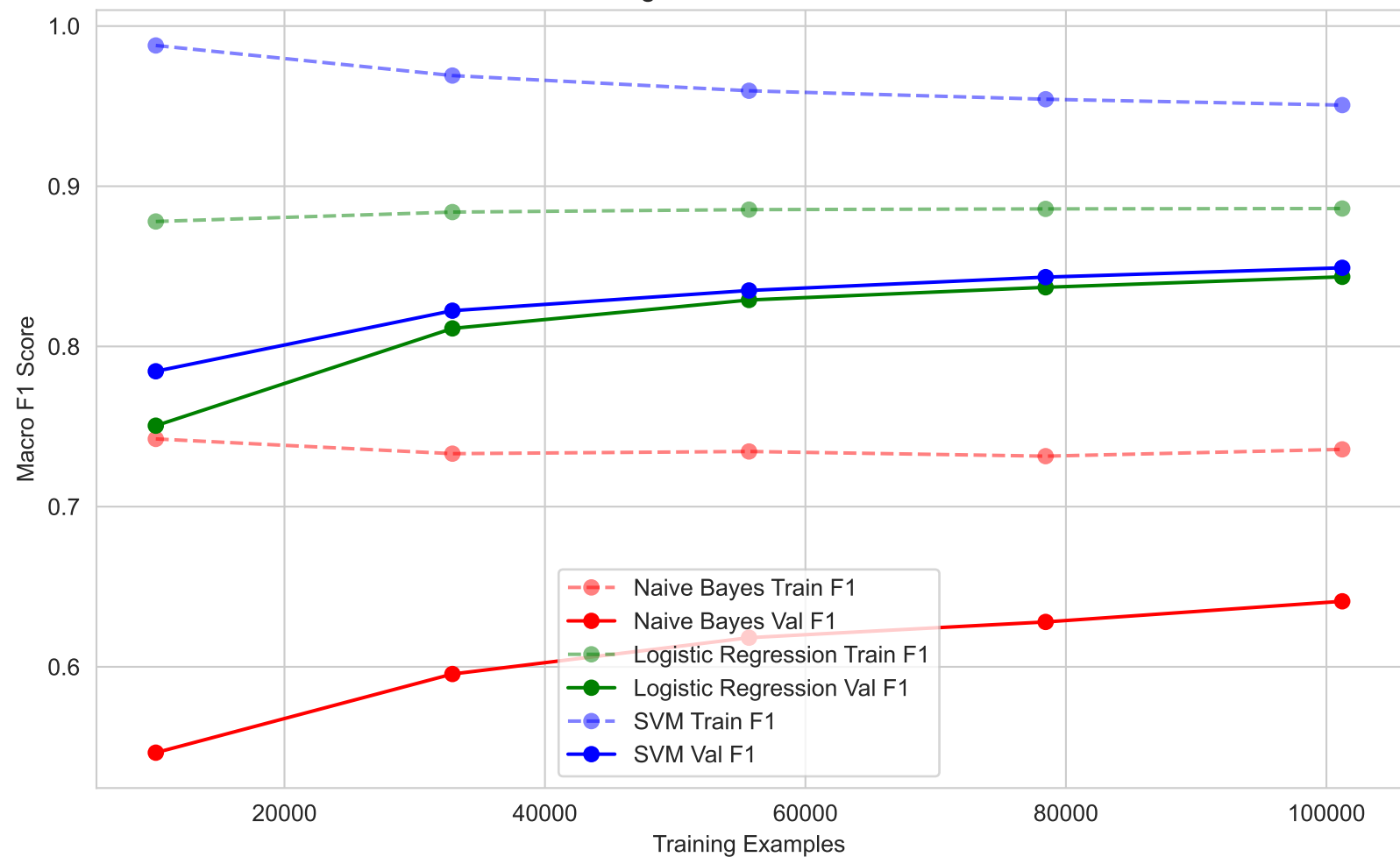
F1 Learning Curves: LR vs NB vs SVM
