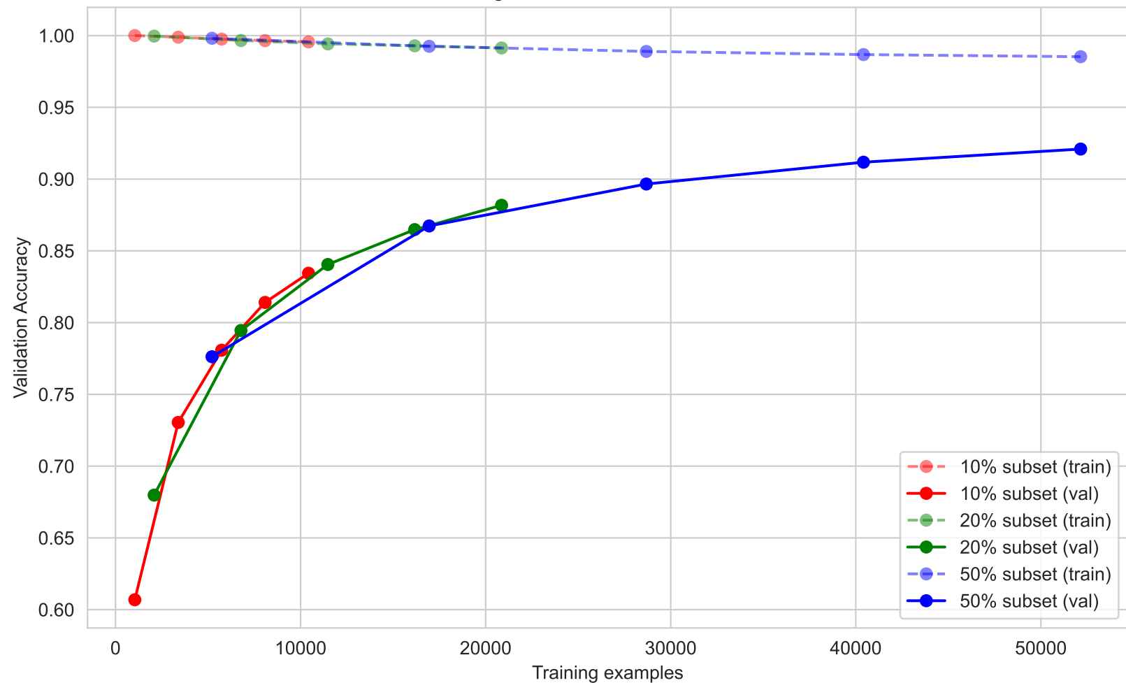
SVM Learning Curve for 10%, 20%, 50% subsets
