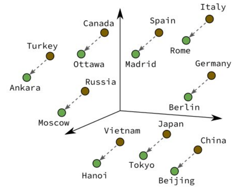
Country-Capital
