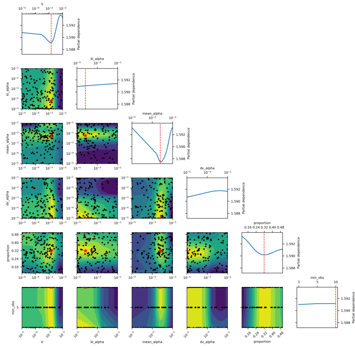
Partial dependence plots for hyperparameter tuning
