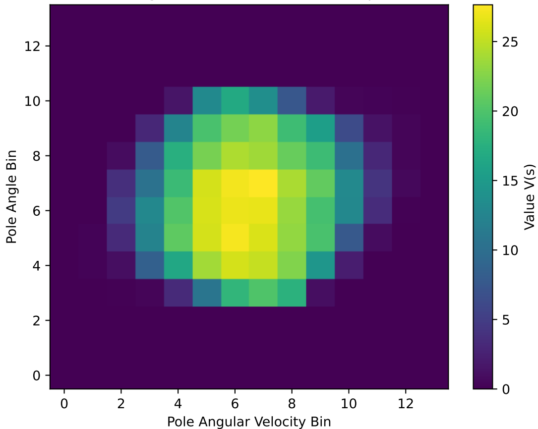
Q-Learning — Value Function Heatmap (b=7)
