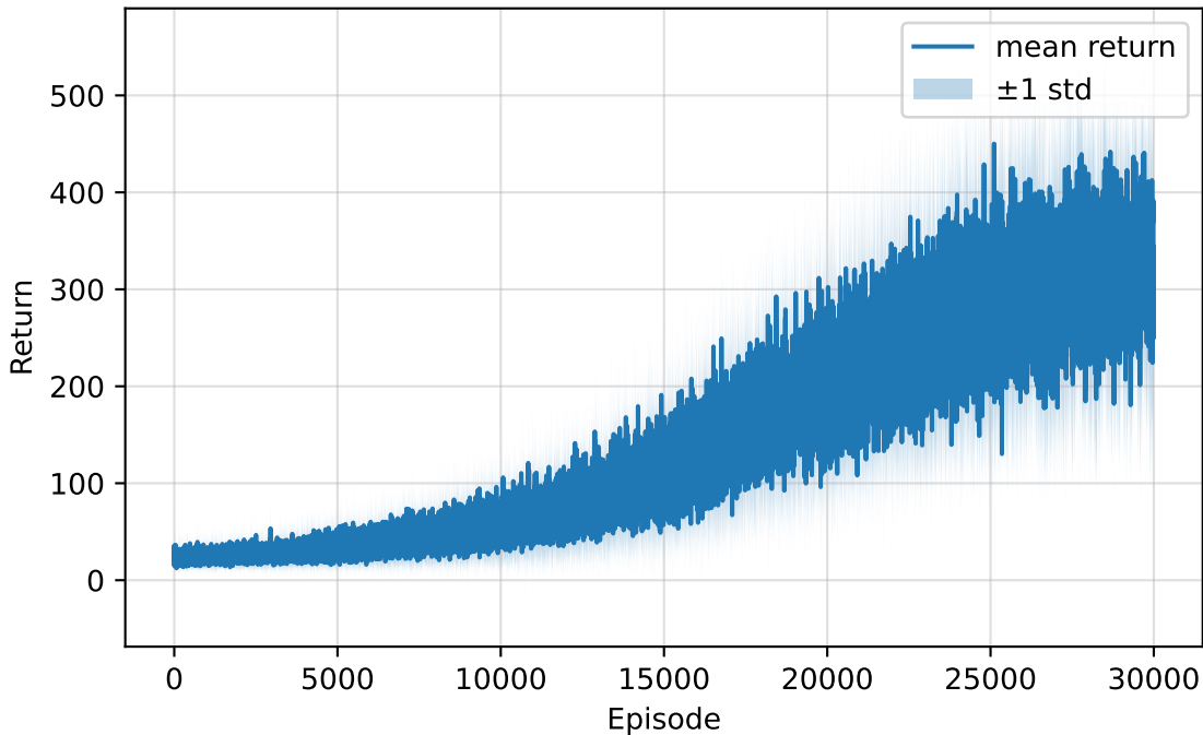
SARSA CartPole — Stability Across Seeds (b=7)
