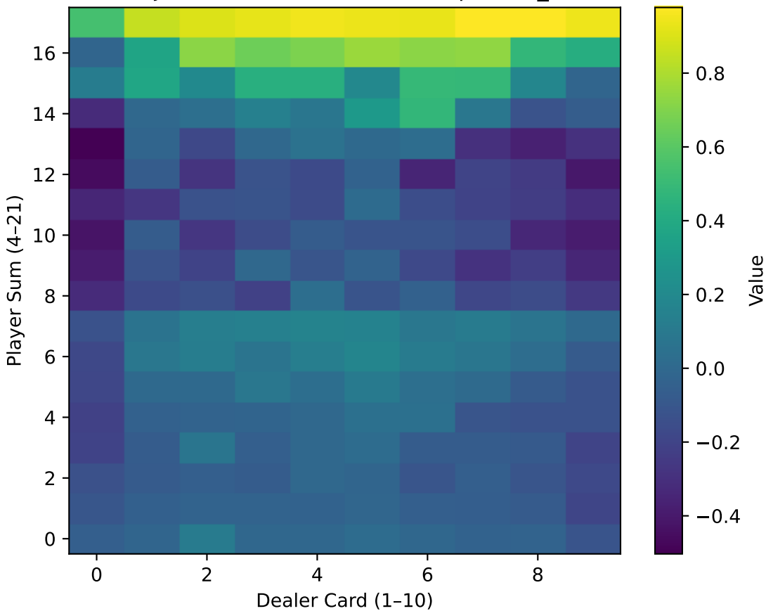
Blackjack SARSA: Final Value Map (max_a Q)
