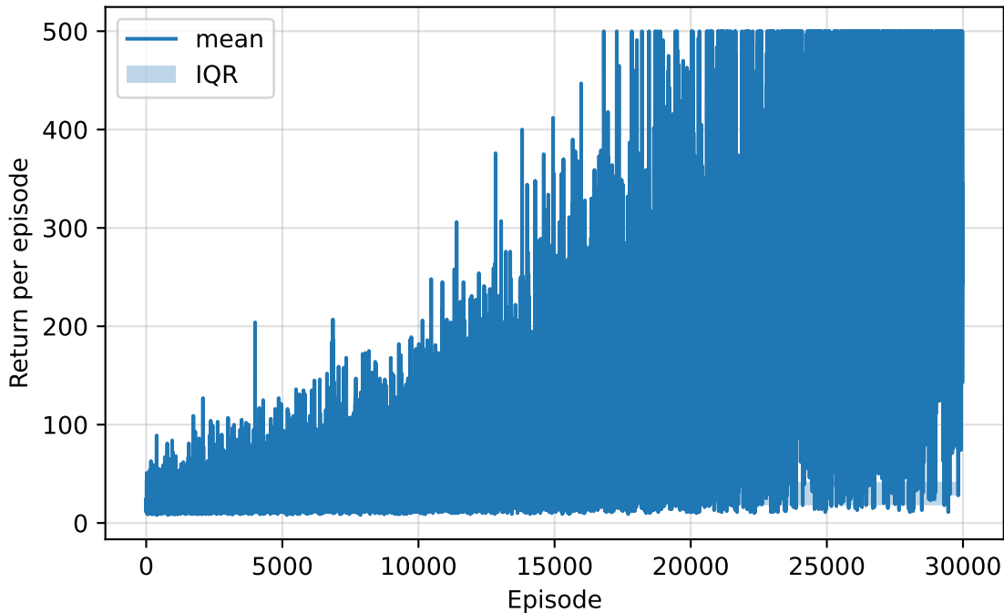
Q-Learning CartPole — Learning Curve (b=7)
