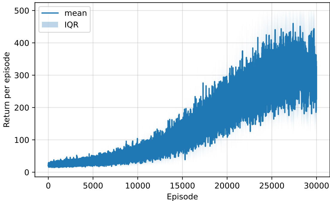
SARSA CartPole — Learning Curve (b=7)
