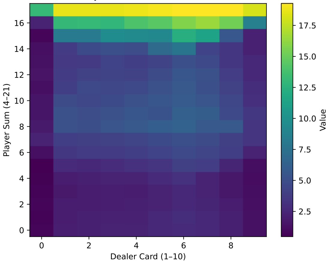
Blackjack PI: Final Value Function
