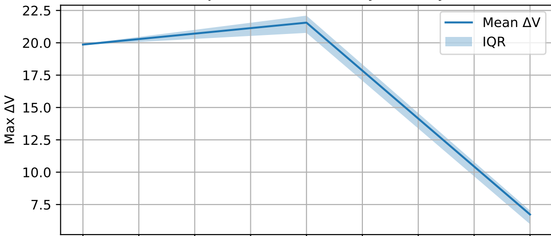
Blackjack PI: \Delta V and Policy Stability
