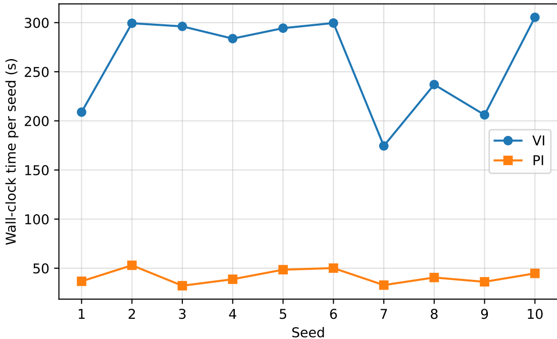
Wall-clock time vs seed (base n_bins=9)
