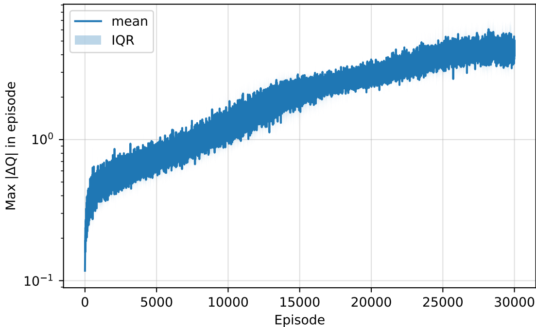
SARSA CartPole — \Delta Q per Episode (b=7)
