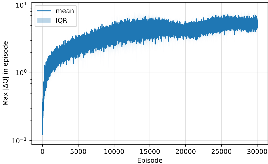
Q-Learning CartPole — \Delta Q per Episode (b=7)
