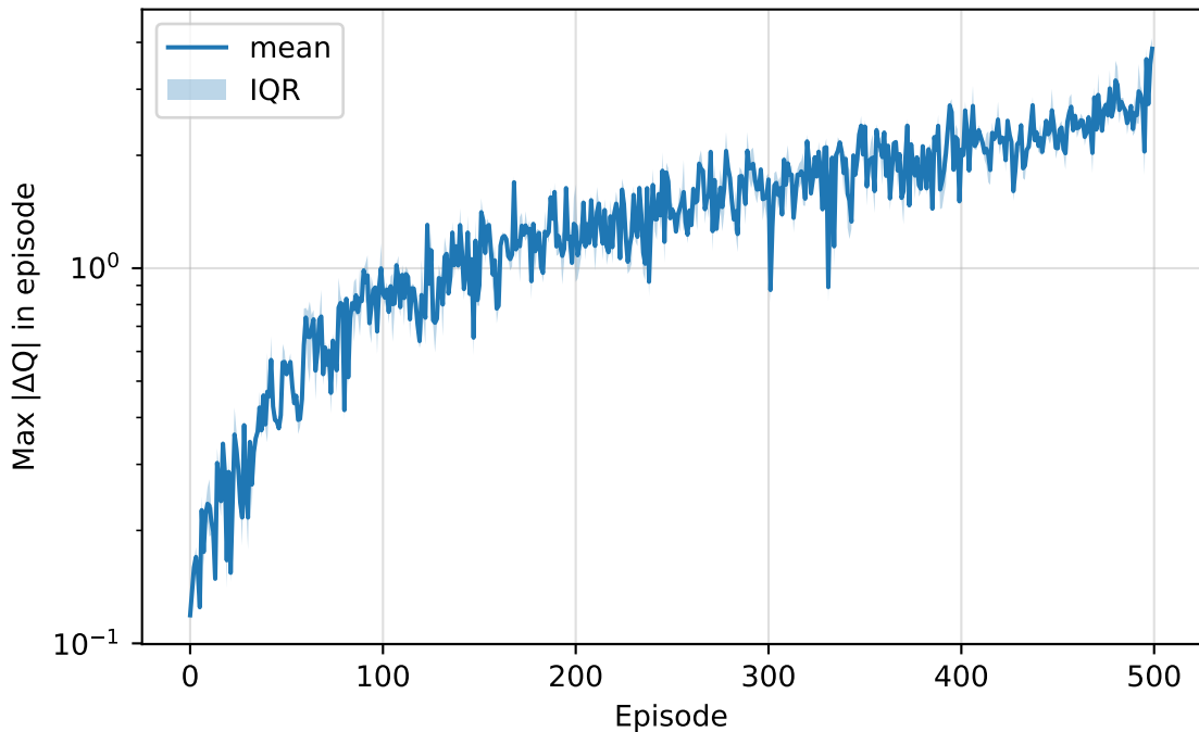
SARSA CartPole — \Delta Q per Episode (b=3)
