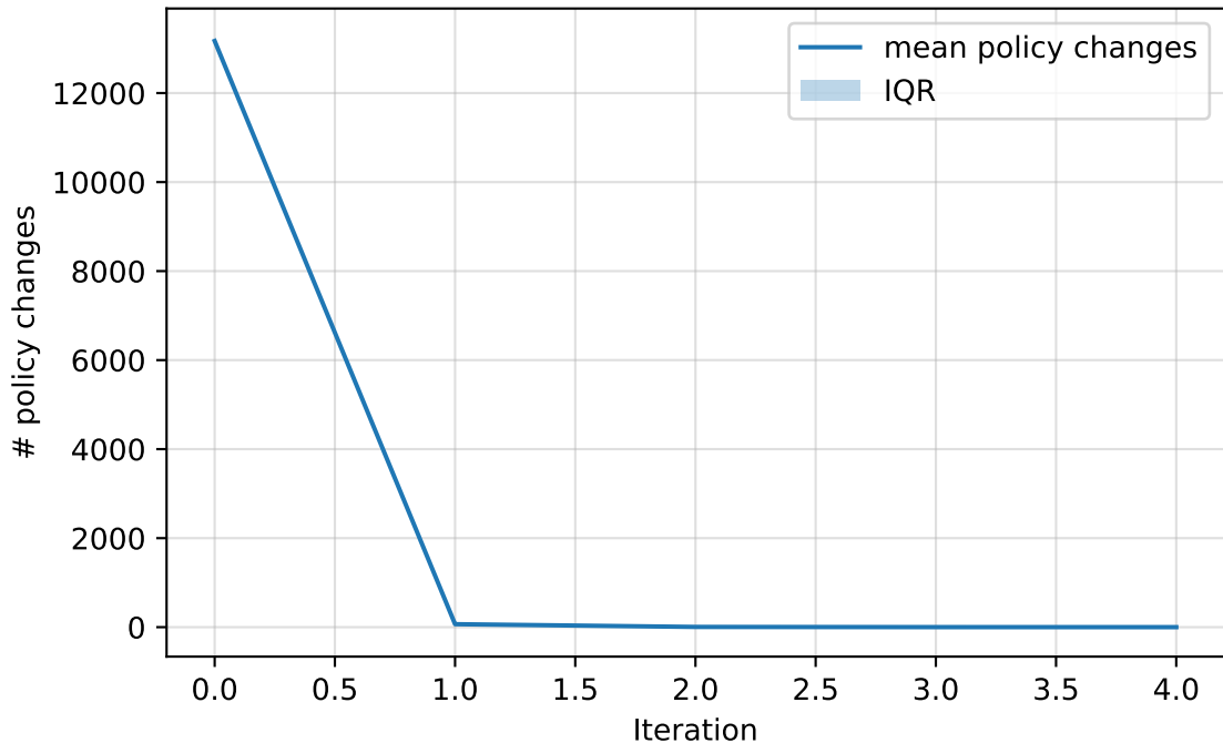
CartPole PI Policy Changes (base n_bins=9)
