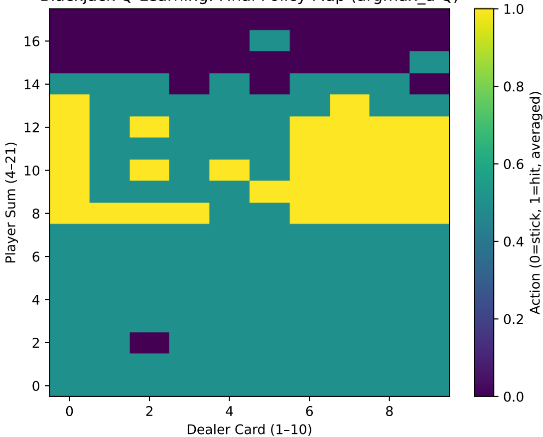
Blackjack Q-Learning: Final Policy Map (argmax_a Q)
