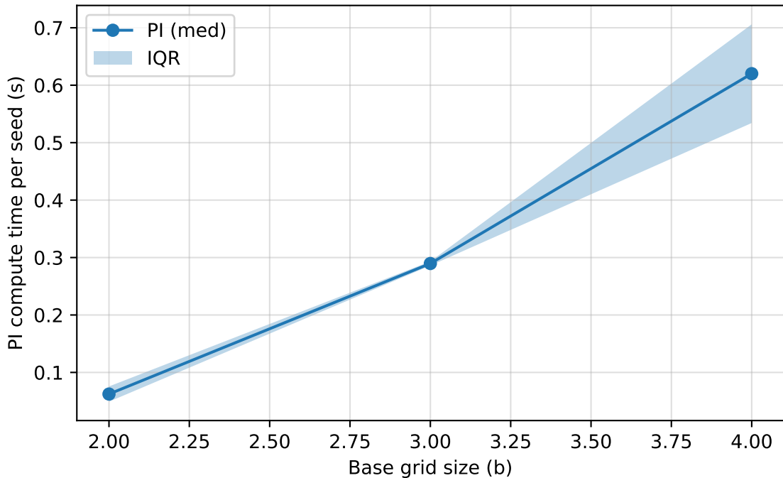
Grid size vs PI Compute Time (median + IQR)
