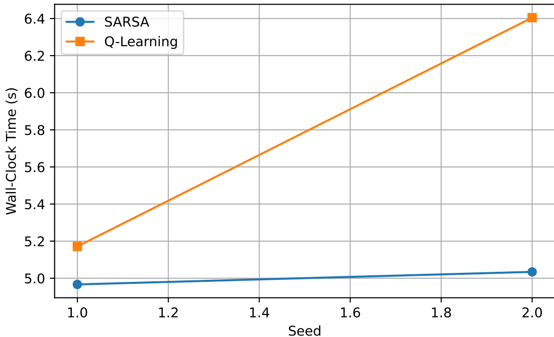
Blackjack: Wall-Clock Time per Seed (SARSA vs Q-Learning)
