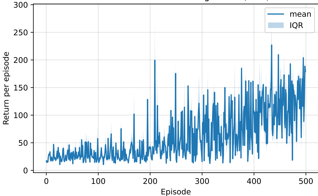
SARSA CartPole — Learning Curve (b=3)
