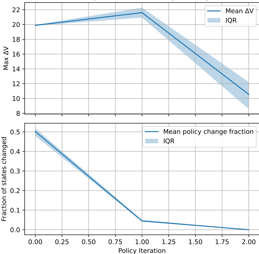
Blackjack PI: \Delta V and Policy Stability
