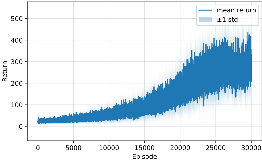
Q-Learning CartPole — Stability Across Seeds (b=7)
