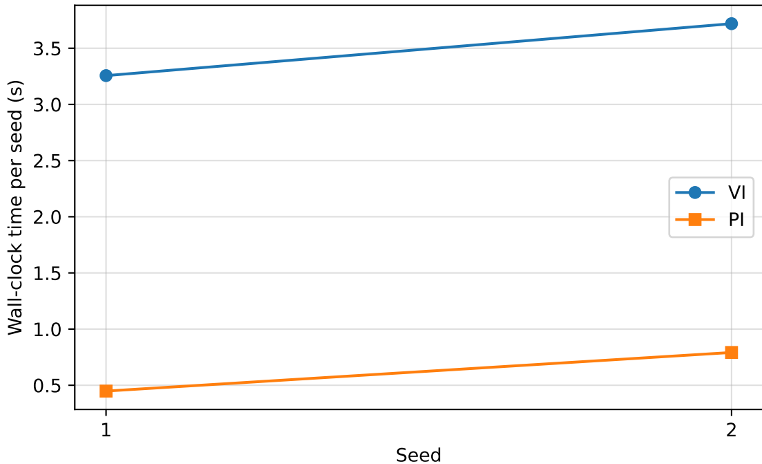
Wall-clock time vs seed (base n_bins=4)
