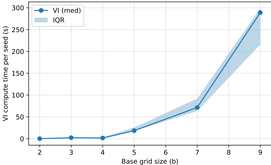
Grid size vs VI Compute Time (median + IQR)
