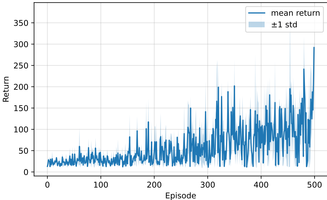
SARSA CartPole — Stability Across Seeds (b=3)
