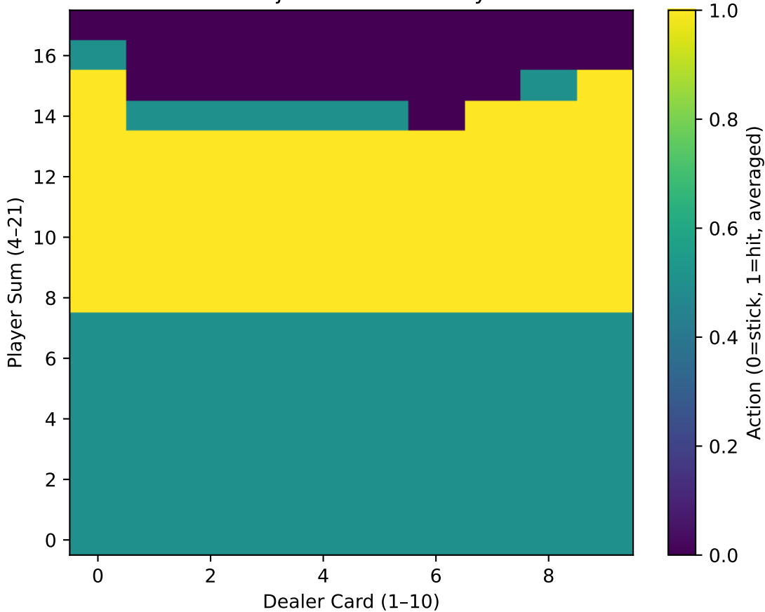
Blackjack PI: Final Policy
