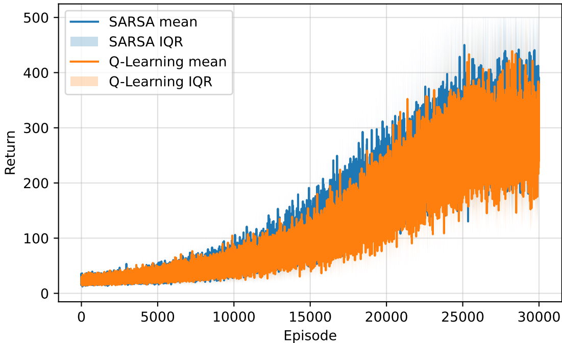
SARSA vs Q-Learning — Learning Curve (b=7)
