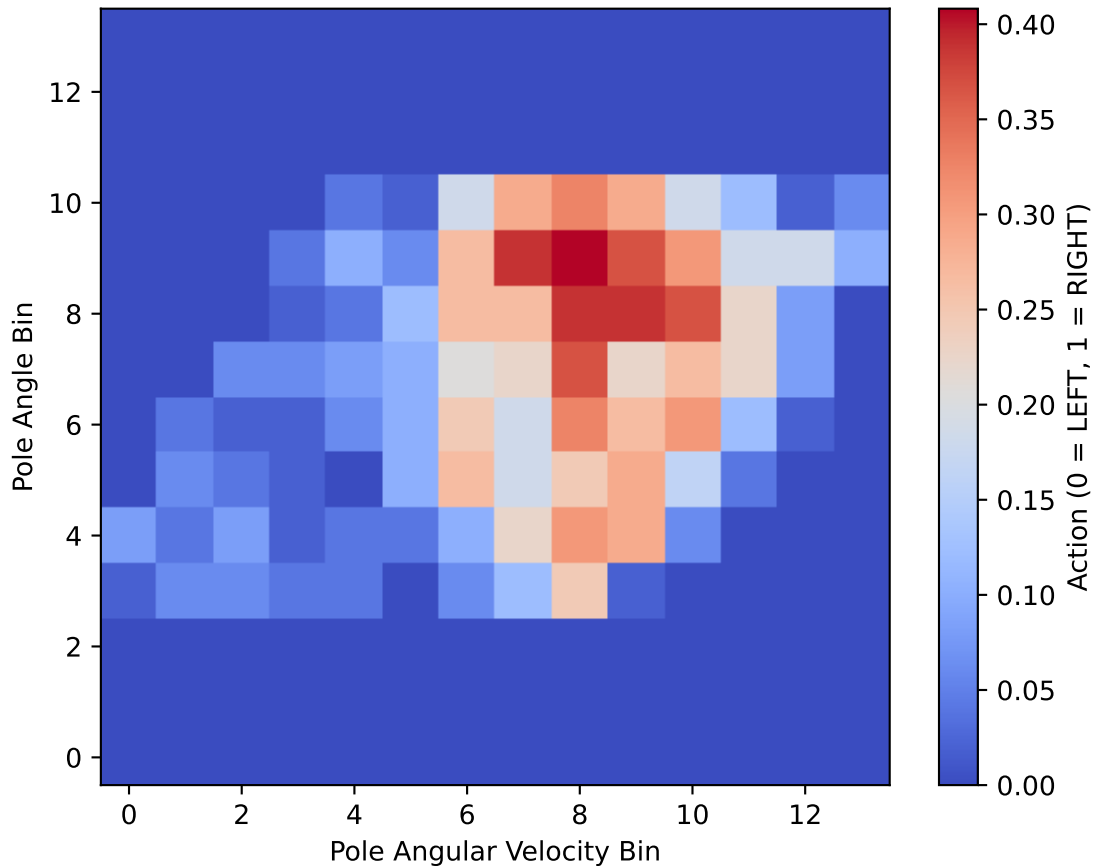
Q-Learning — Policy Heatmap (b=7)
