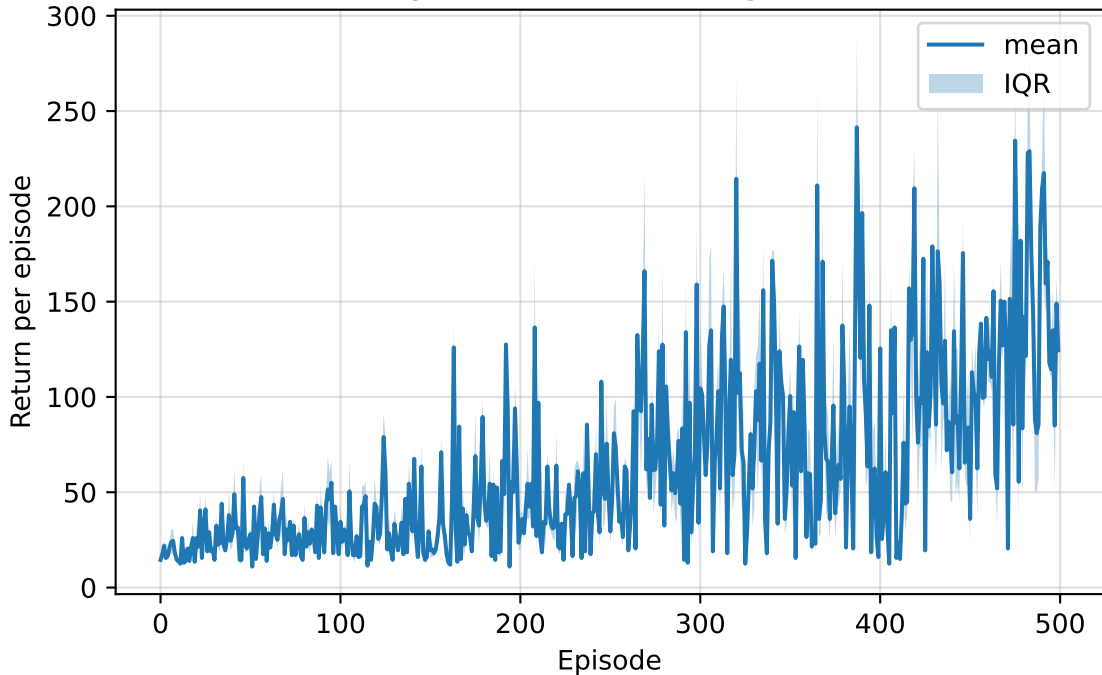
Q-Learning CartPole — Learning Curve (b=3)
