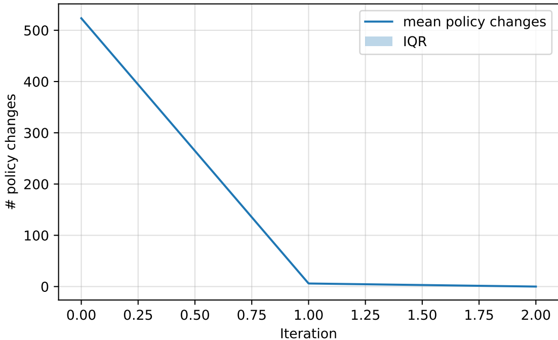
CartPole PI Policy Changes (base n_bins=4)
