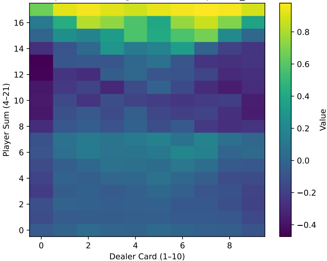
Blackjack Q-Learning: Final Value Map (max_a Q)
