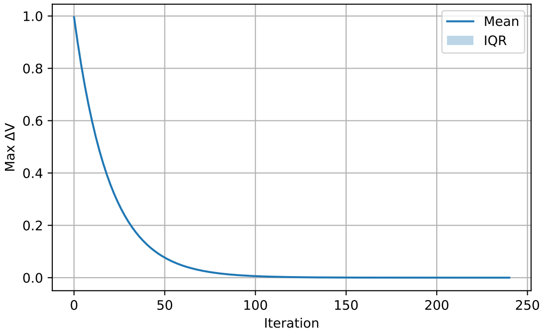
Blackjack VI: \Delta V vs Iterations
