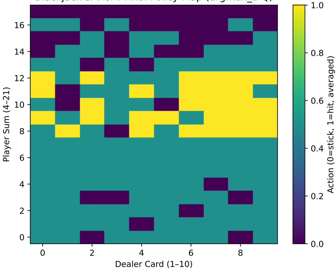
Blackjack SARSA: Final Policy Map (argmax_a Q)
