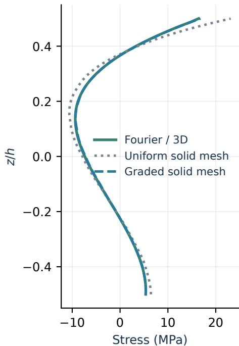
(a) Near-edge \sigma_{xx}
