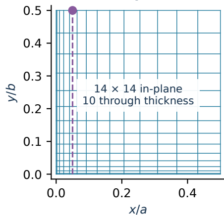
(c) Graded quarter mesh
