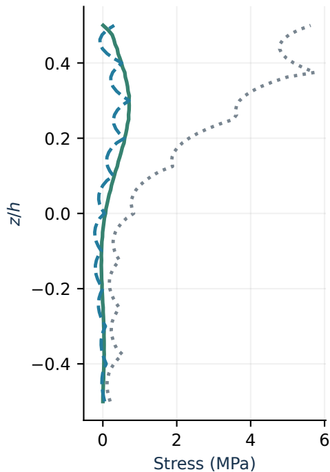
(b) Near-edge \sigma_{zz}
