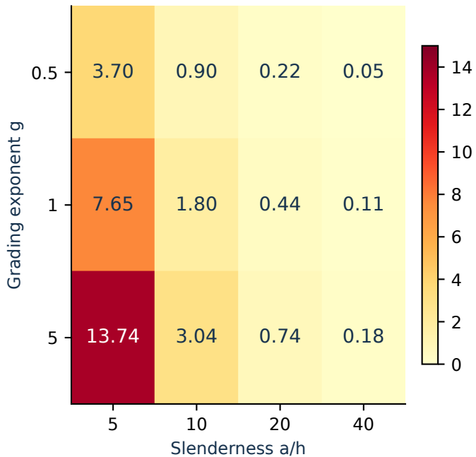
(a) Centre displacement
