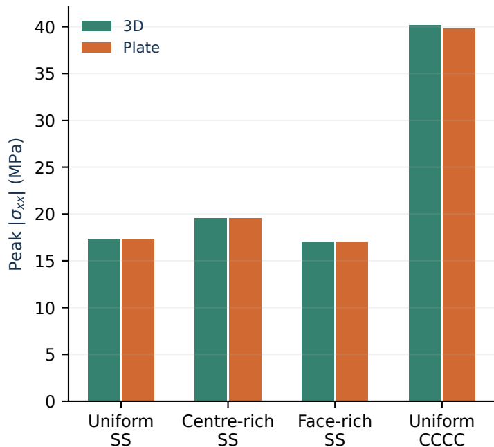
(b) Centre-path peak normal stress
