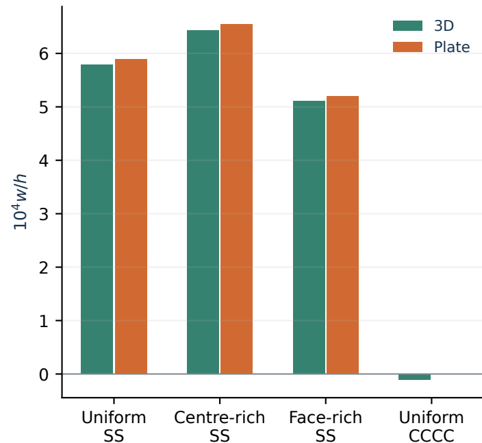
(a) Centre displacement
