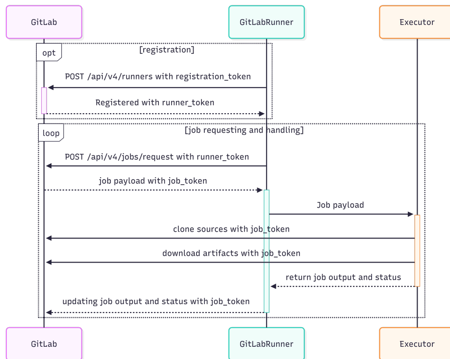
Figure 5.3: Sequence diagram of registration, polling, and execution flow.
