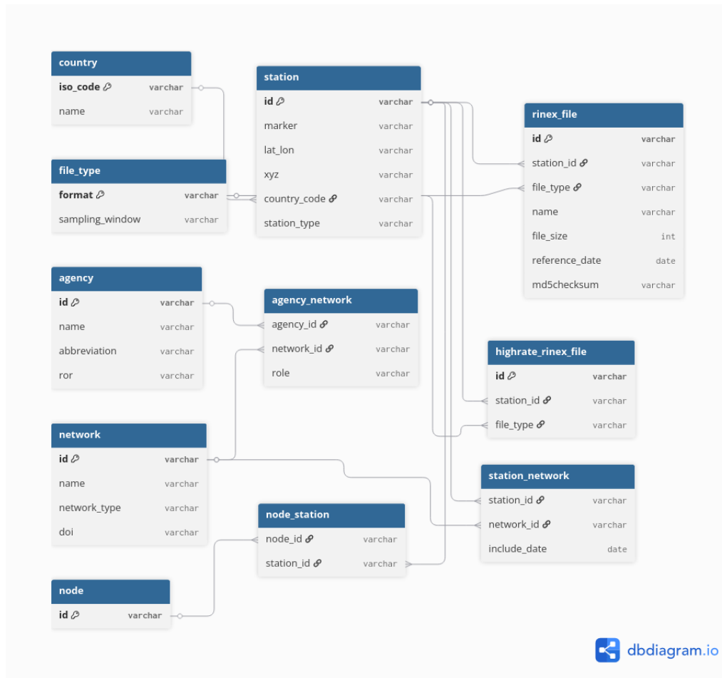
Figure 5.2: Simplified view of the core EPOS data model.
