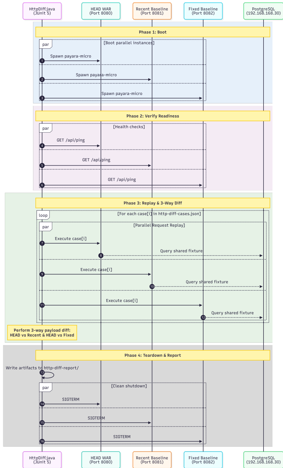
Figure 5.4: Phases of HttpDiff.java . The harness orchestrates boot, verification, parallel replay, and teardown.
