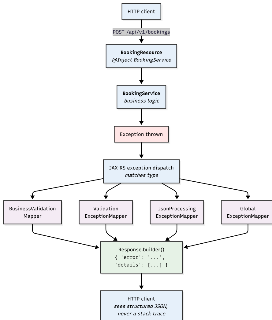
Figure 4.1: The CDI + JAX-RS exception-handling flow JSON error body.
