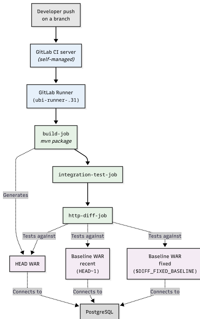
Figure 4.2: Overall architecture of the differential testing framework.
