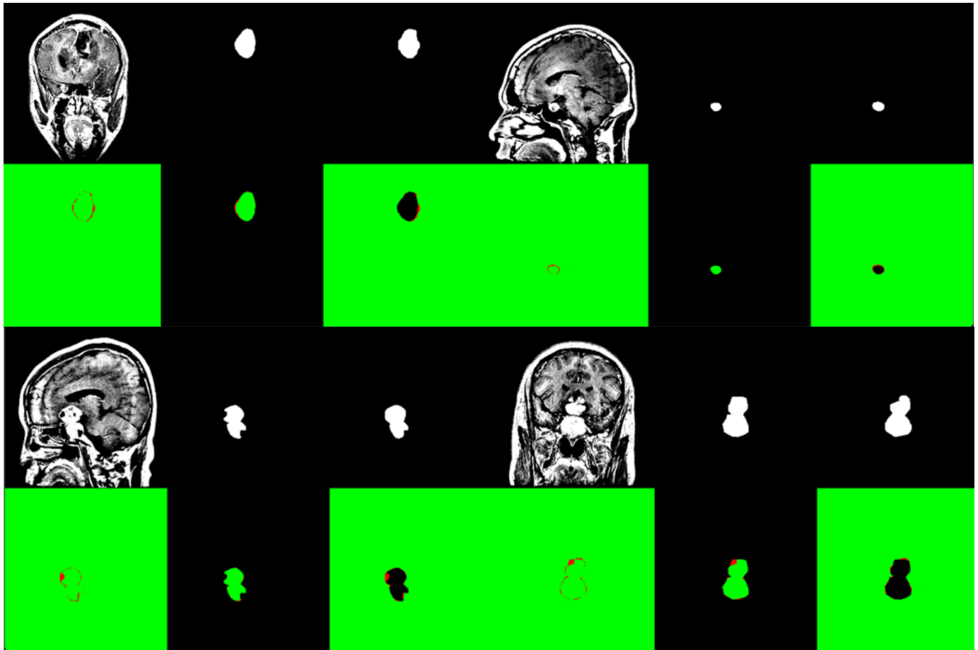
Fig. 3. Examples of our models segmentation masks with correct vs. incorrect pixel comparison.
