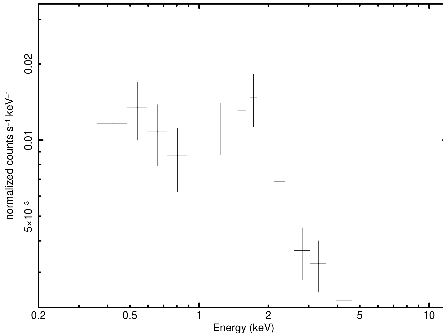
Source 1 minus background (P0921180101M1S001SRSPEC0001)
