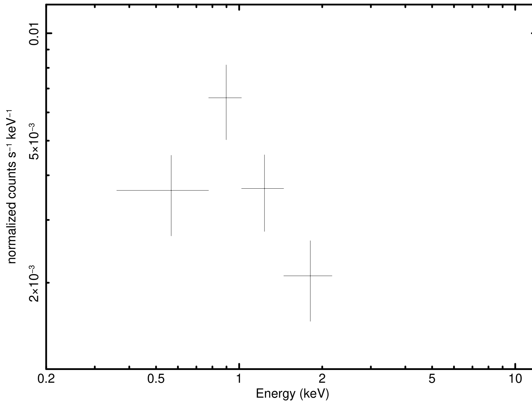
Source 7 minus background (P0921180101M1S001SRSPEC0007)
