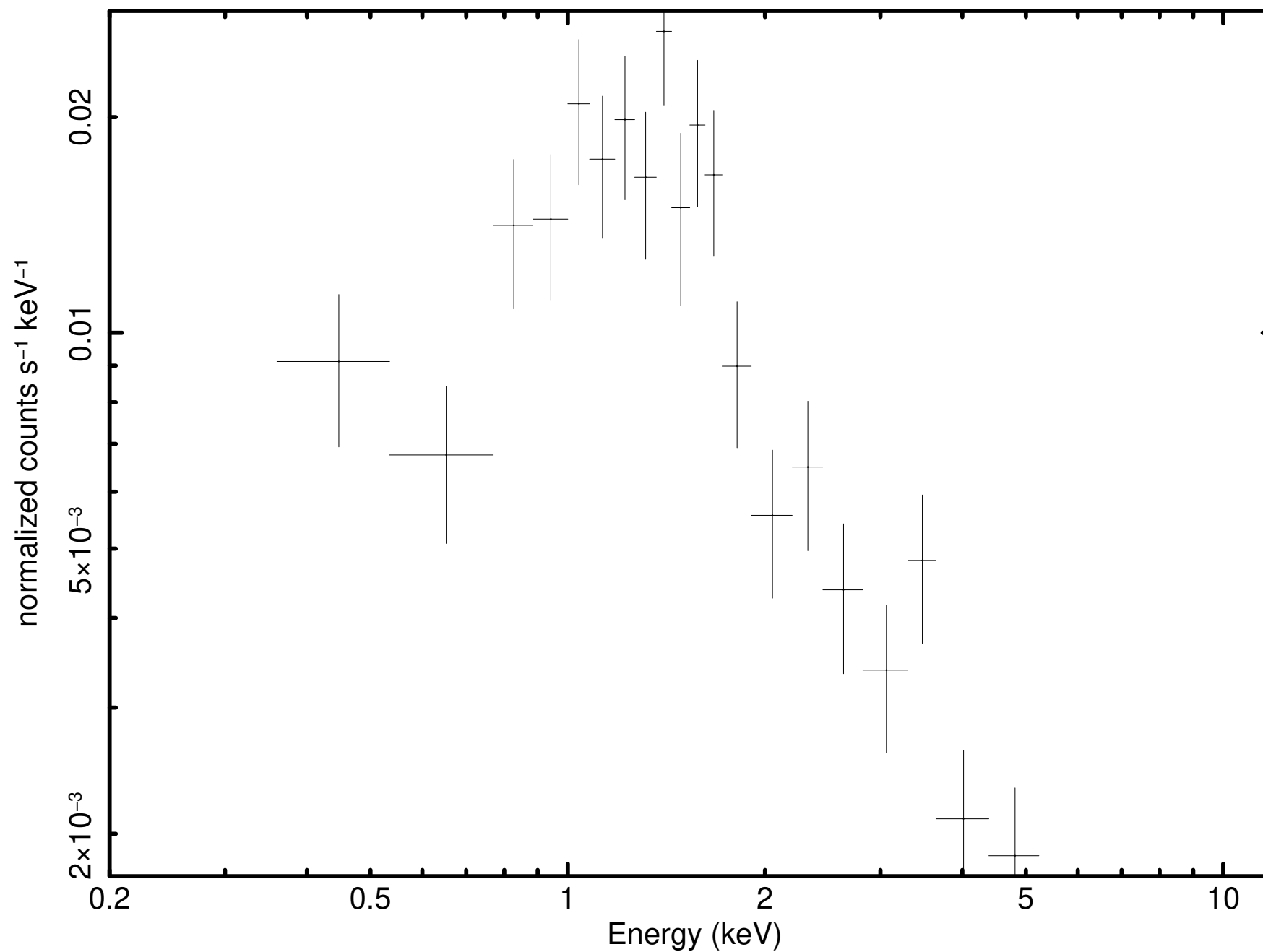
Source 1 minus background (P0921180101M2S002SRSPEC0001)
