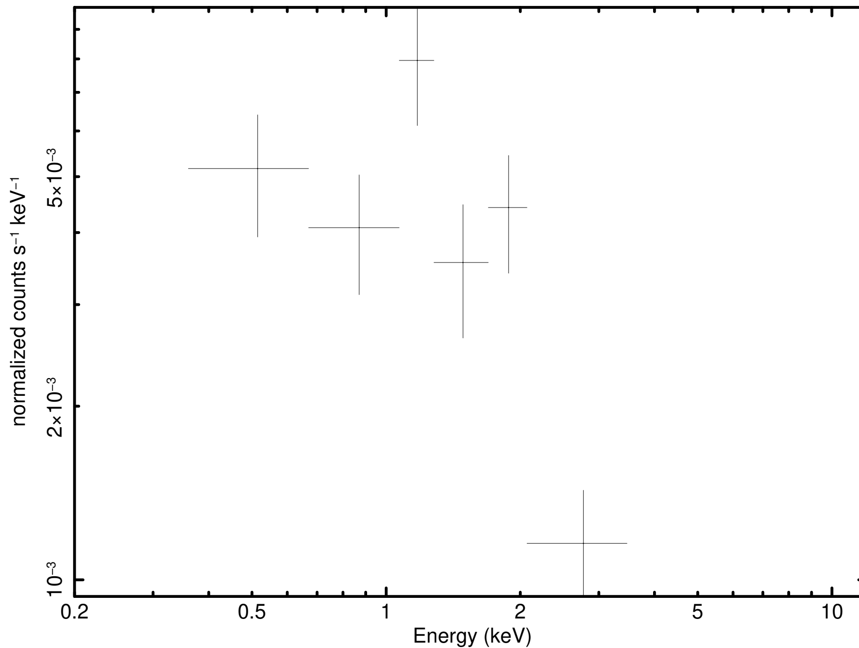
Source 4 minus background (P0921180101M2S002SRSPEC0004)
