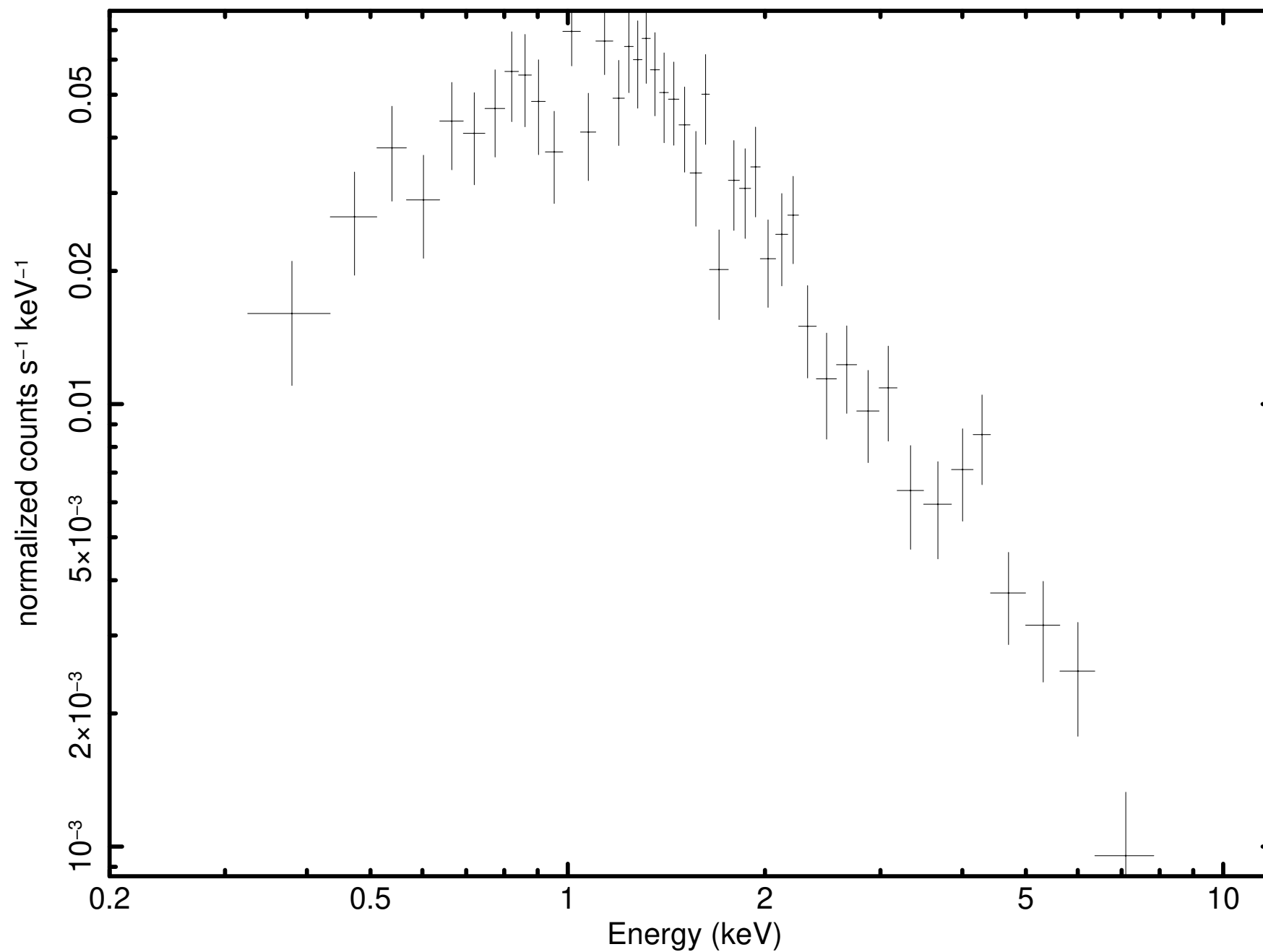
Source 1 minus background (P0921180101PNS003SRSPEC0001)
