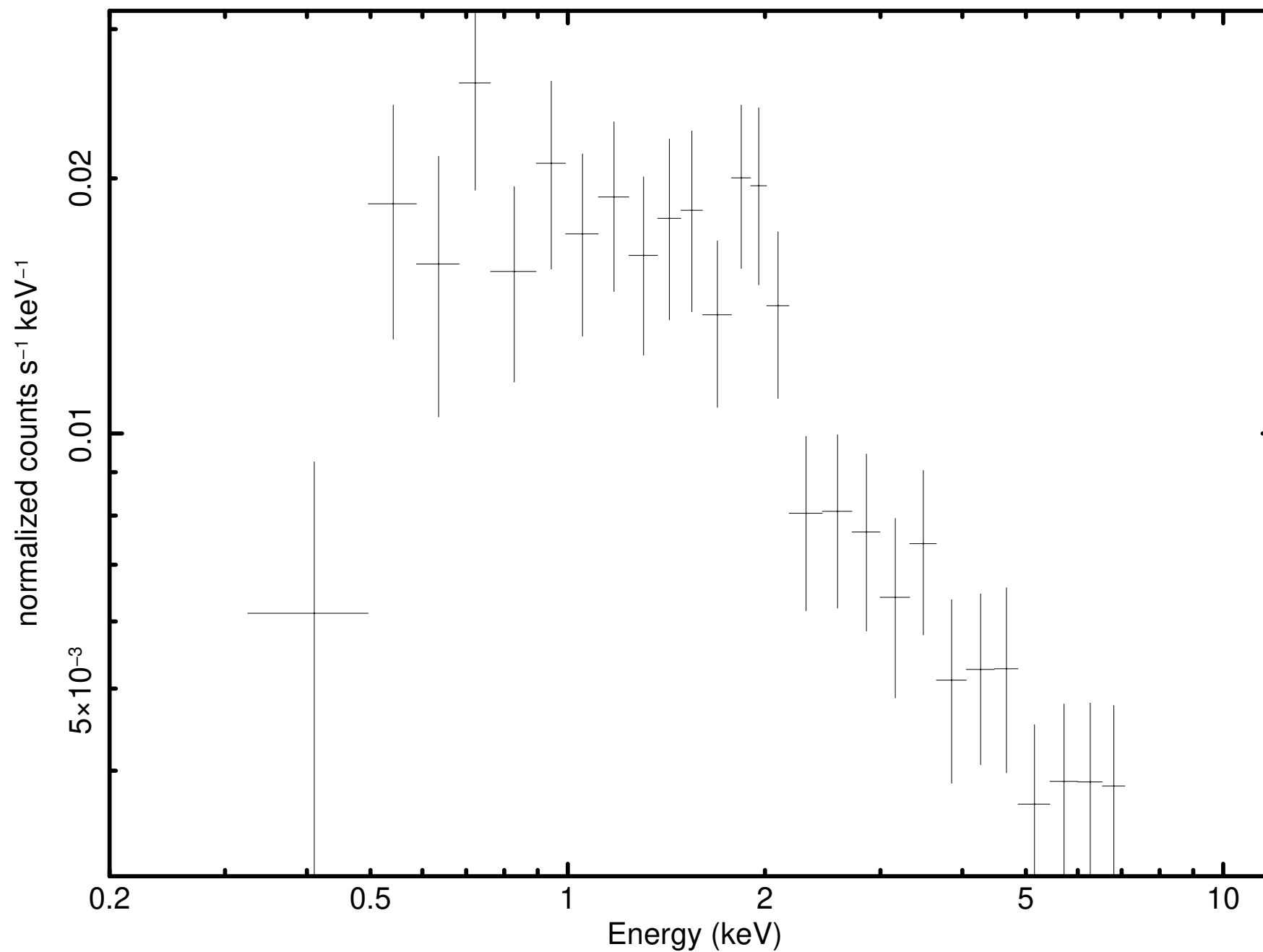
Source 2 minus background (P0921180101PNS003SRSPEC0002)
