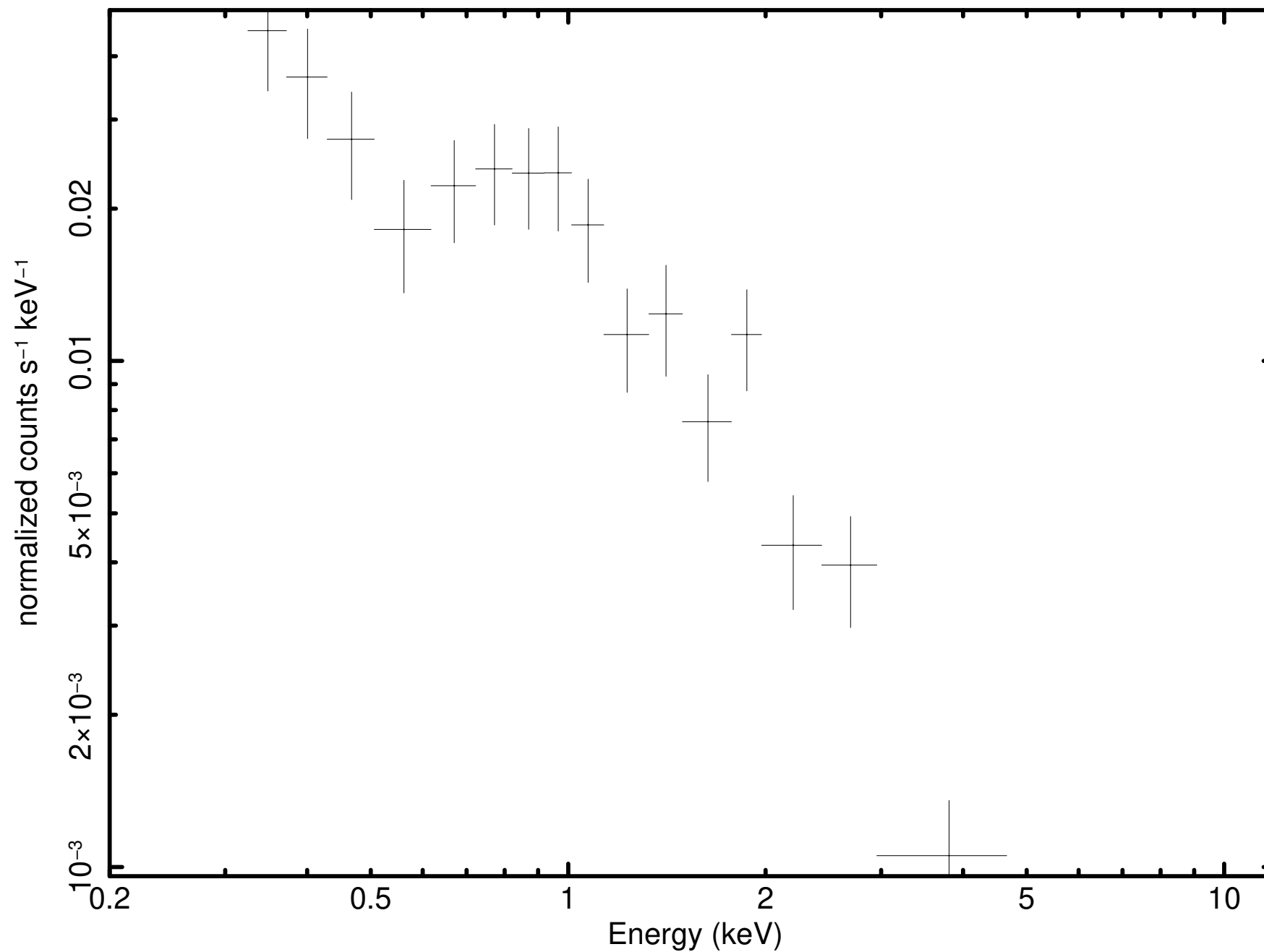
Source 4 minus background (P0921180101PNS003SRSPEC0004)
