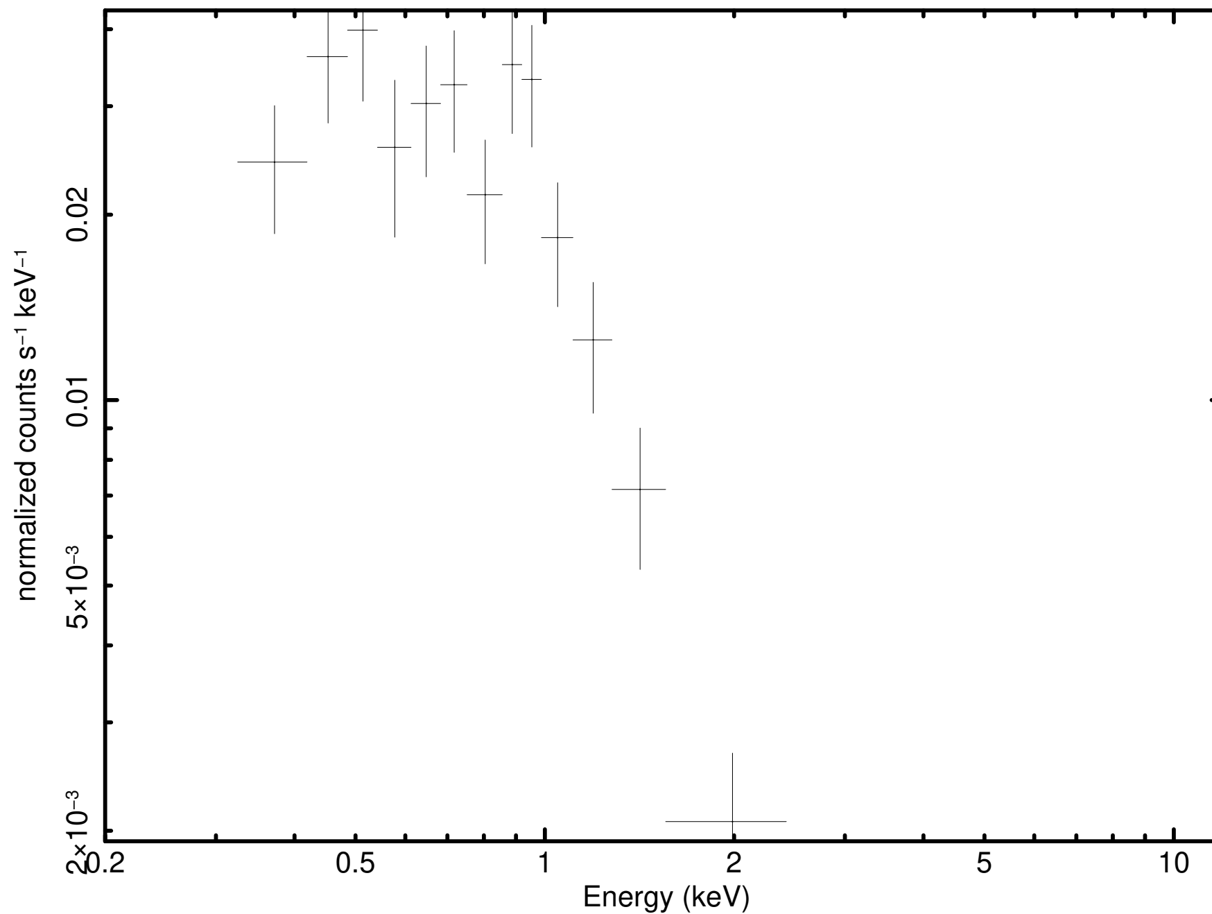
Source 5 minus background (P0921180101PNS003SRSPEC0005)
