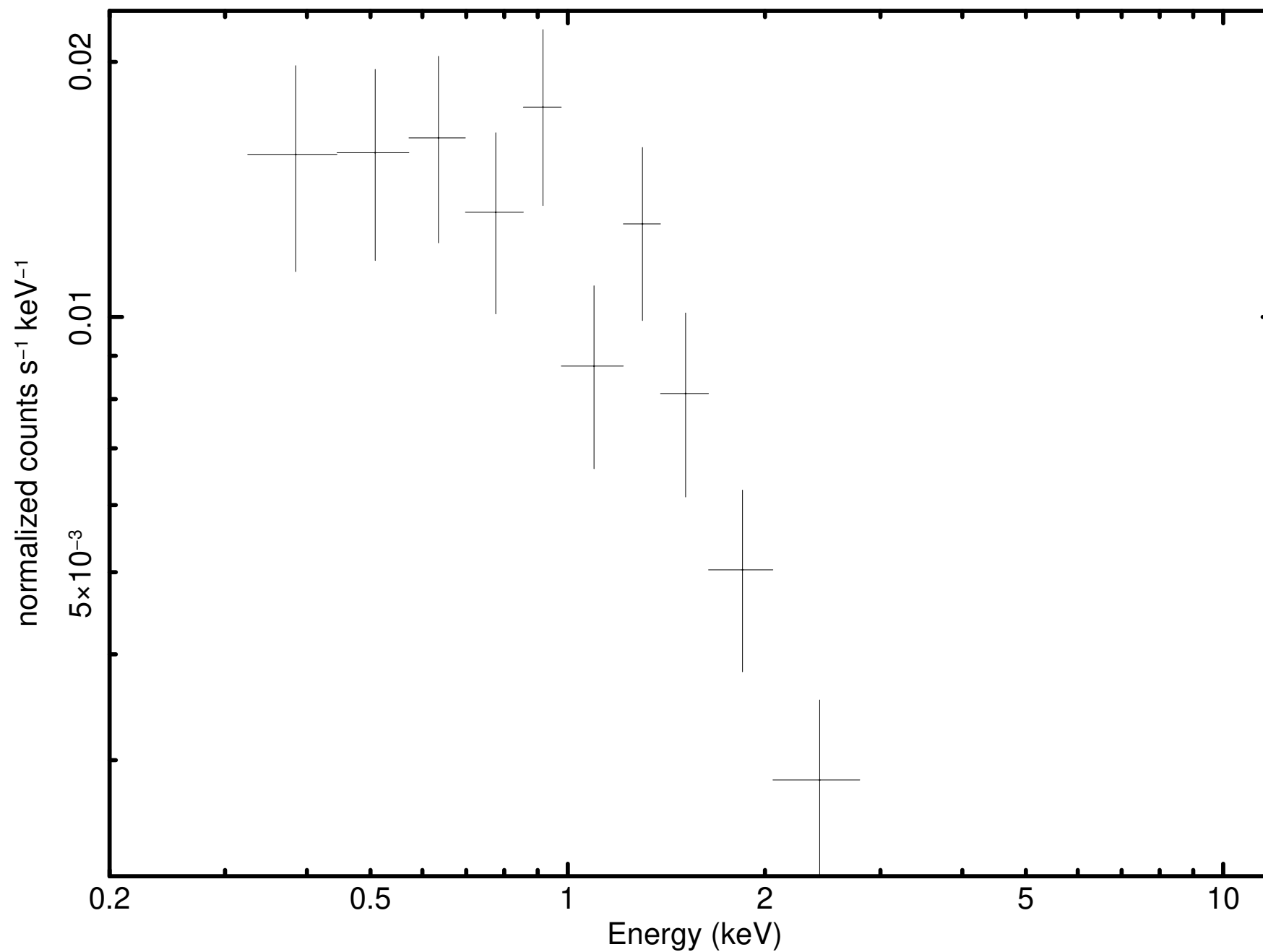
Source 6 minus background (P0921180101PNS003SRSPEC0006)
