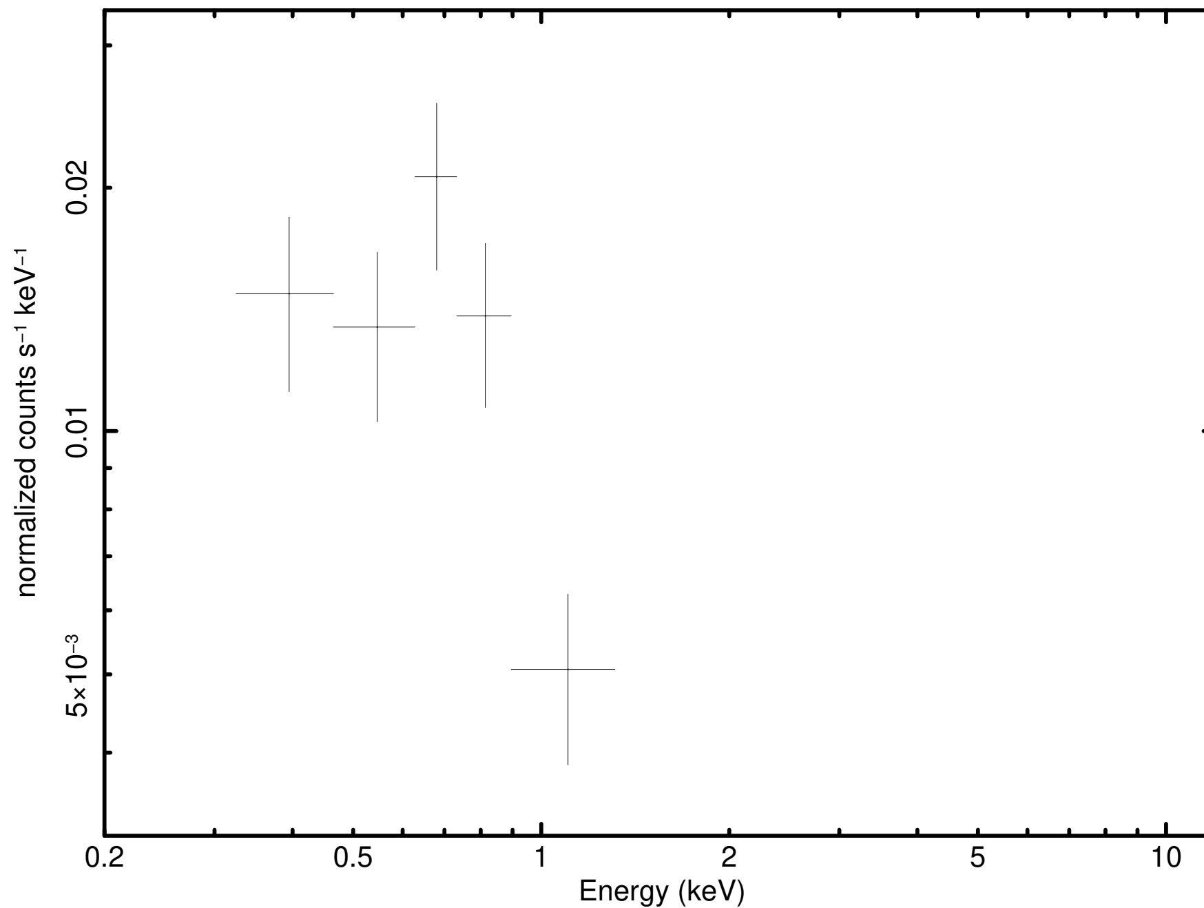
Source 13 minus background (P0921180101PNS003SRSPEC000D)
