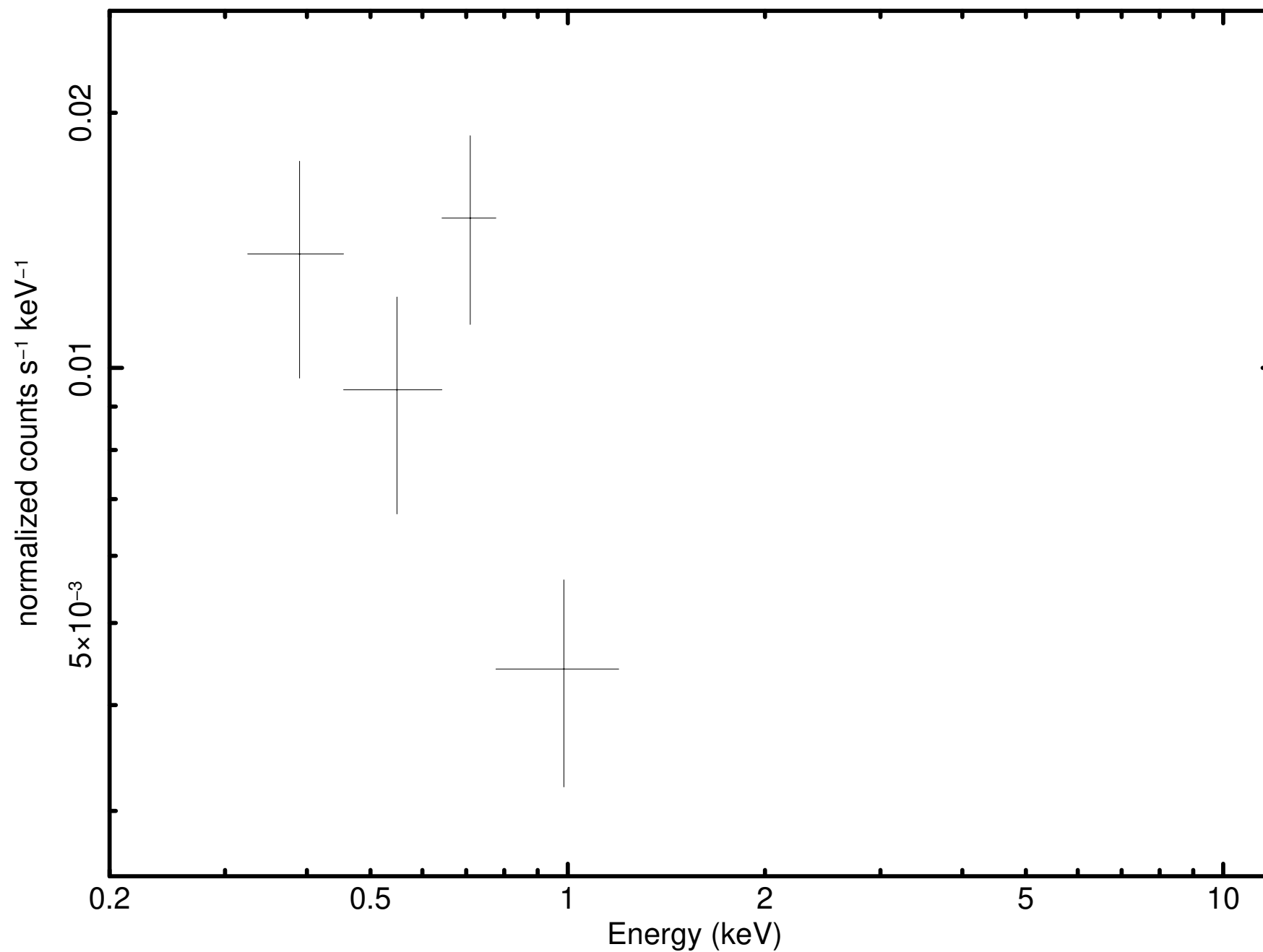
Source 16 minus background (P0921180101PNS003SRSPEC0010)
