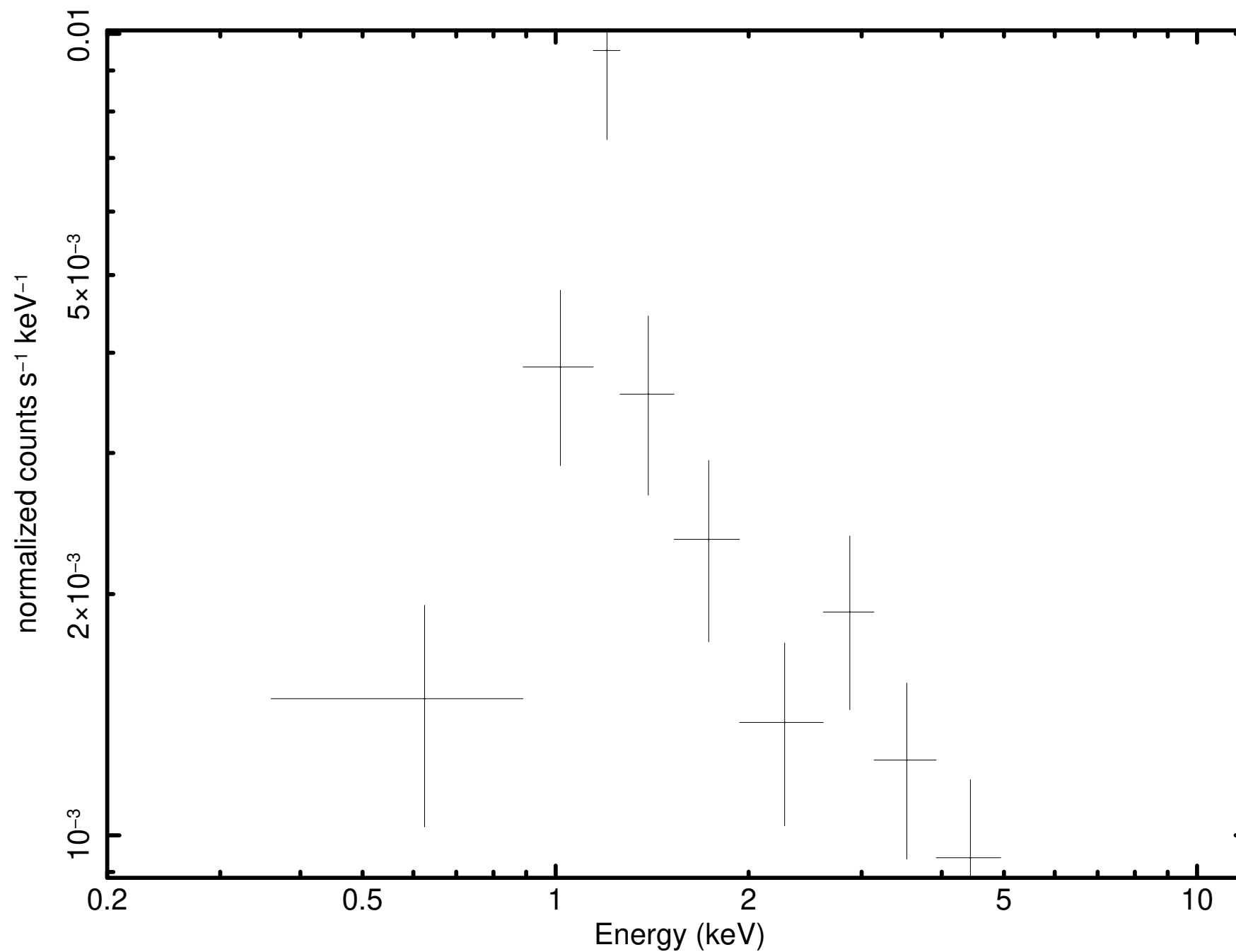
Source 3 minus background (P0921180301M1S001SRSPEC0003)
