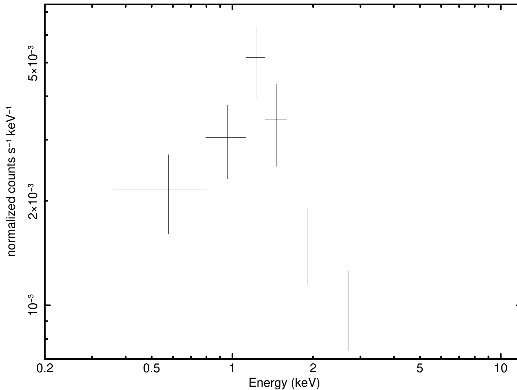
Source 5 minus background (P0921180301M1S001SRSPEC0005)
