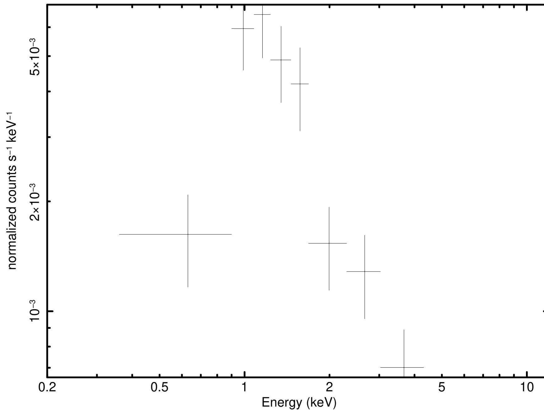
Source 6 minus background (P0921180301M1S001SRSPEC0006)
