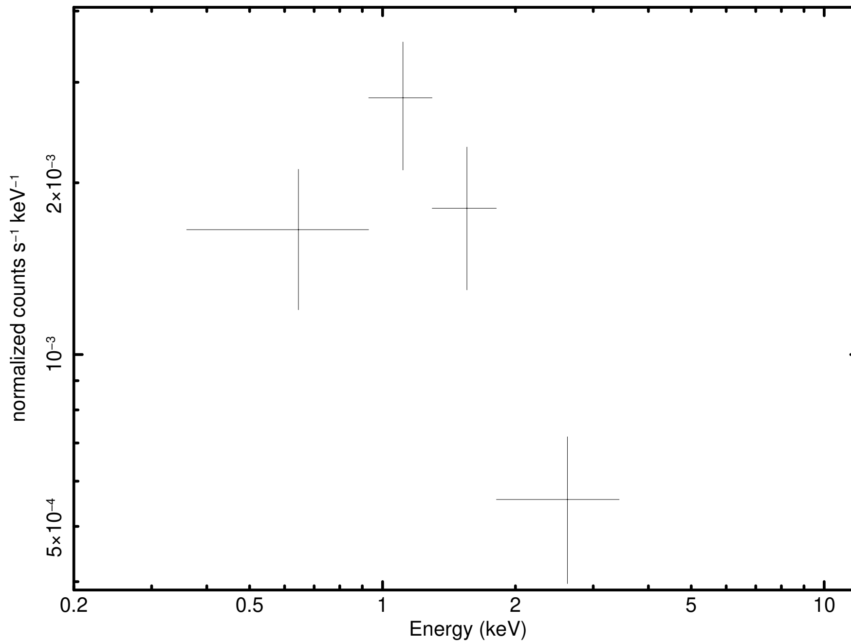
Source 13 minus background (P0921180301M1S001SRSPEC000D)
