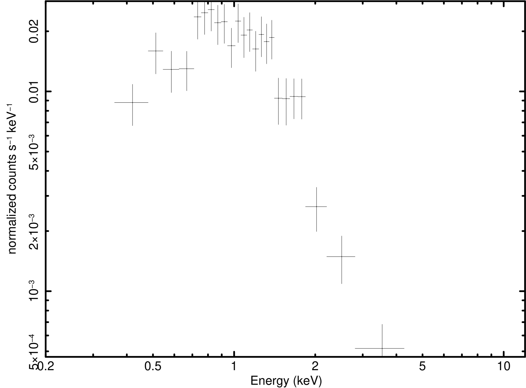
Source 1 minus background (P0921180301M2S002SRSPEC0001)
