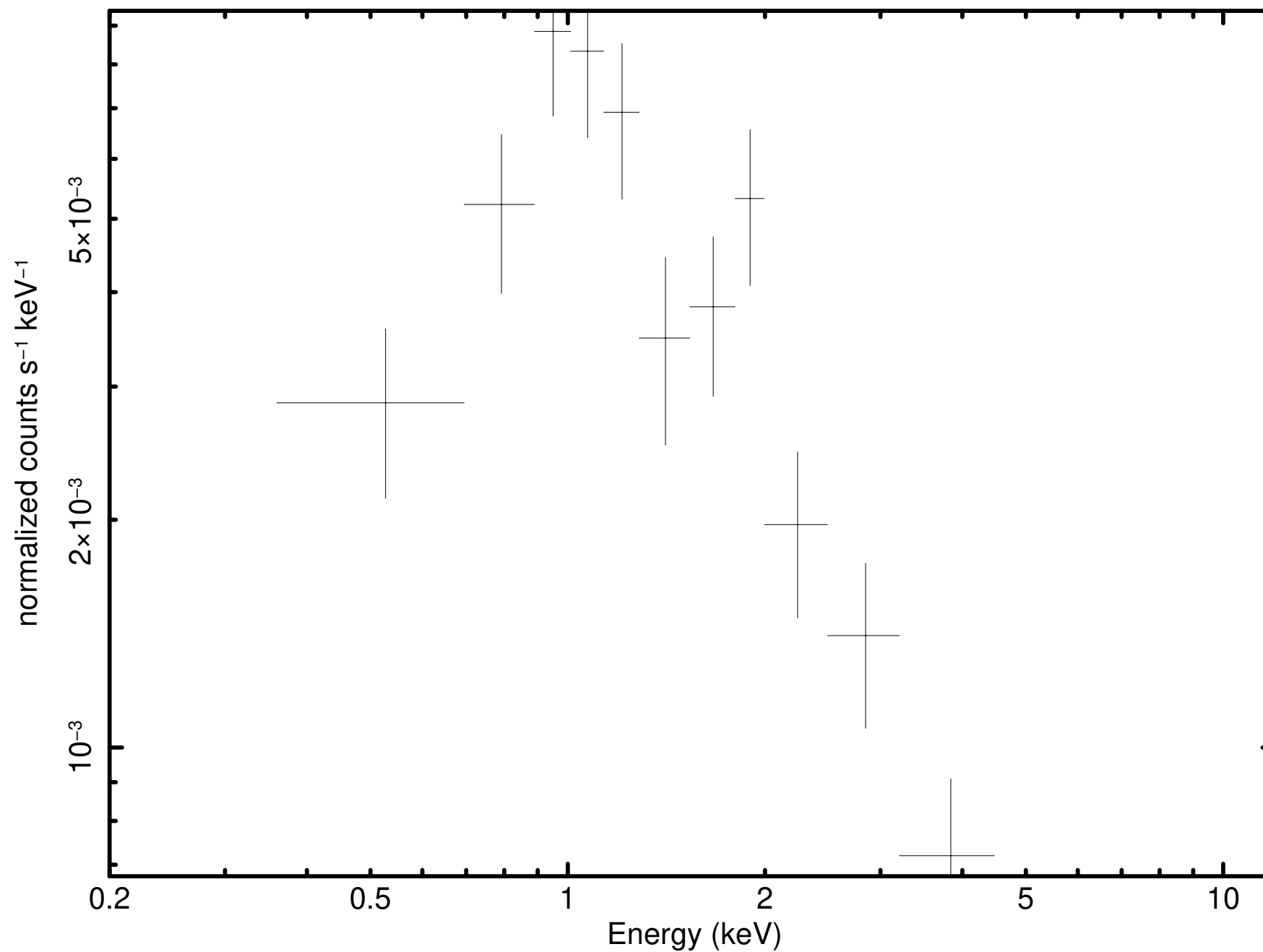
Source 2 minus background (P0921180301M2S002SRSPEC0002)
