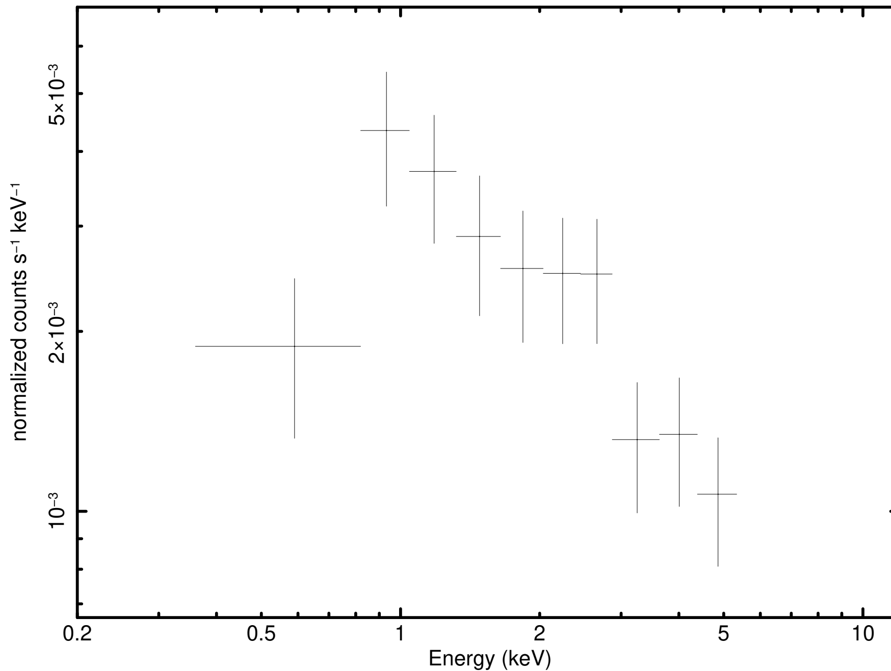
Source 3 minus background (P0921180301M2S002SRSPEC0003)
