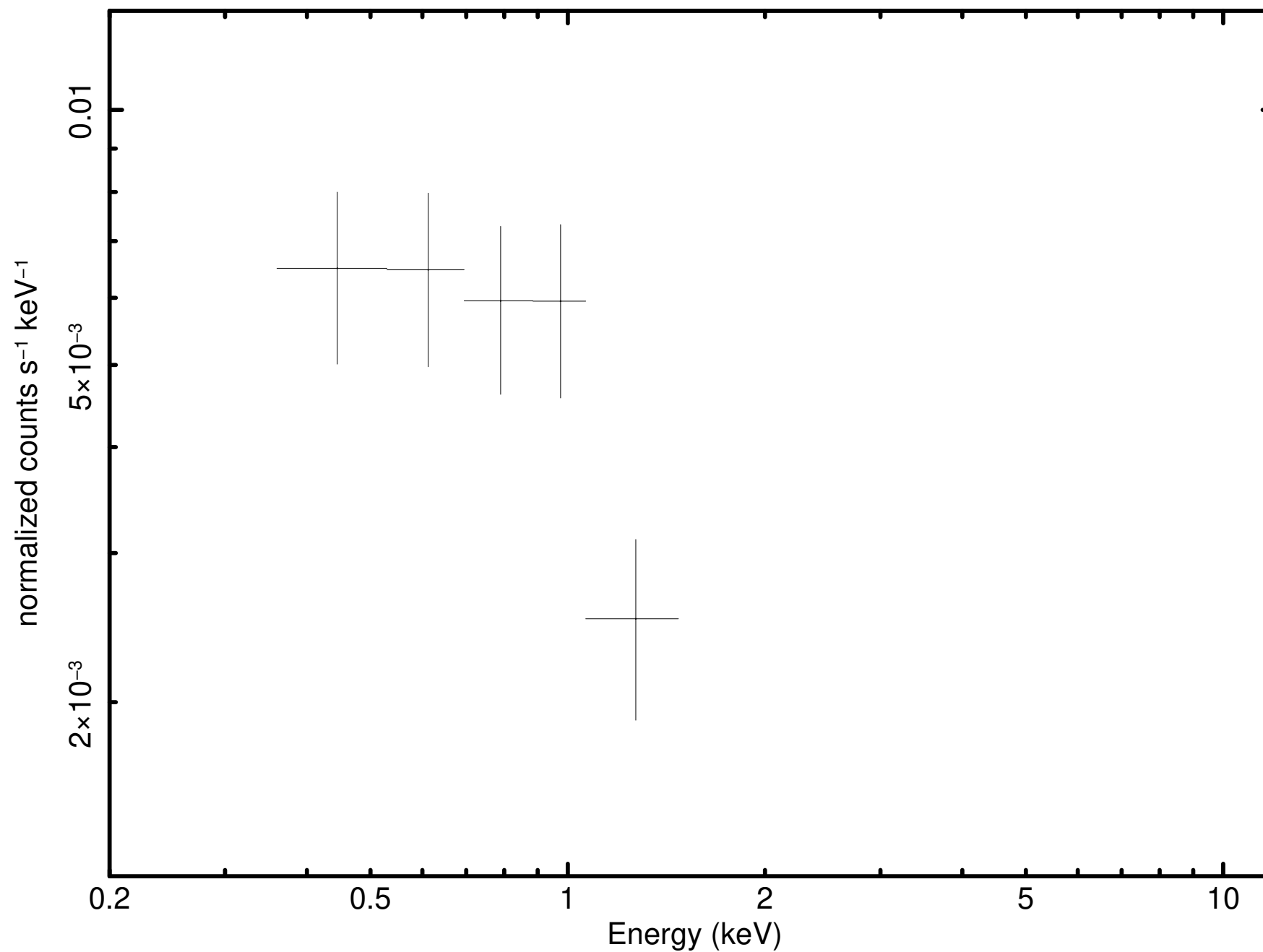
Source 4 minus background (P0921180301M2S002SRSPEC0004)
