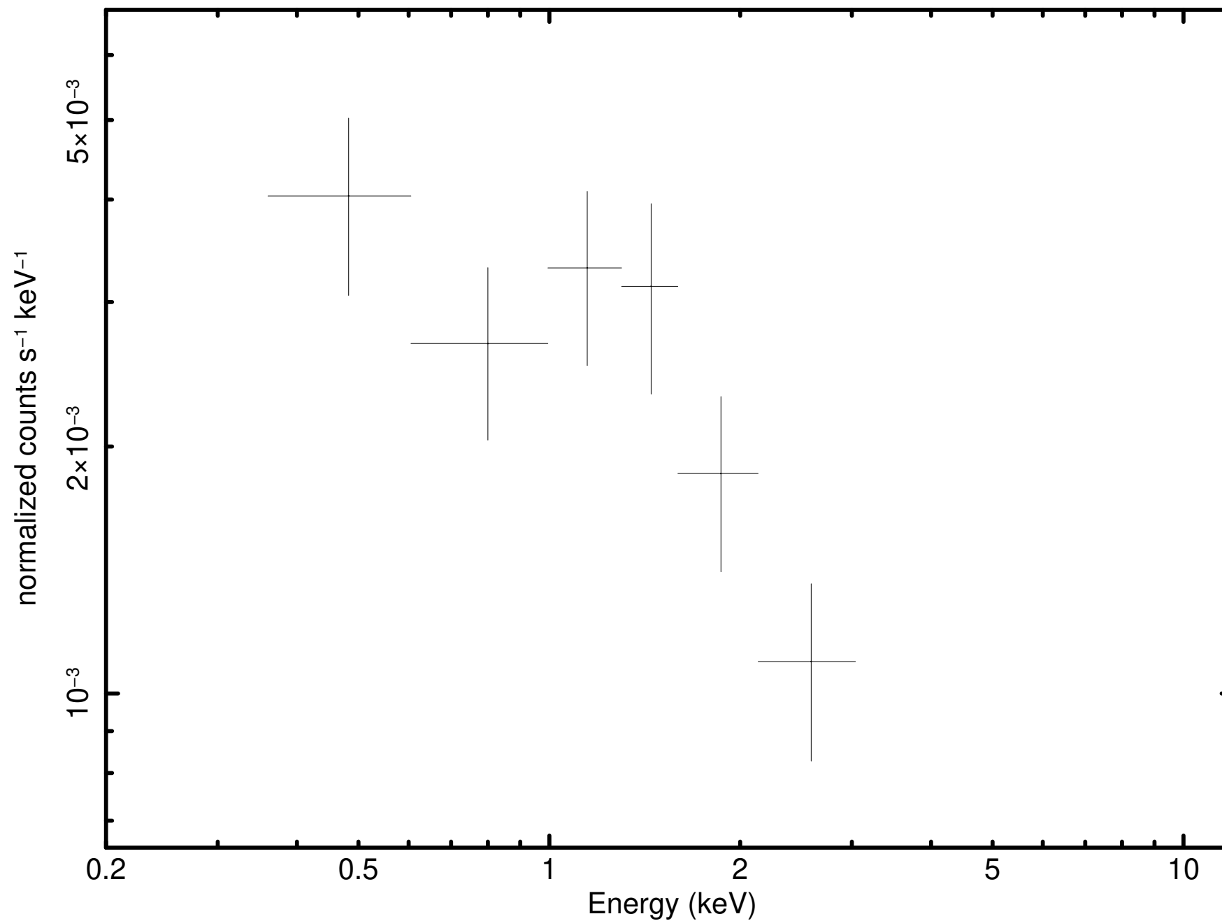
Source 5 minus background (P0921180301M2S002SRSPEC0005)
