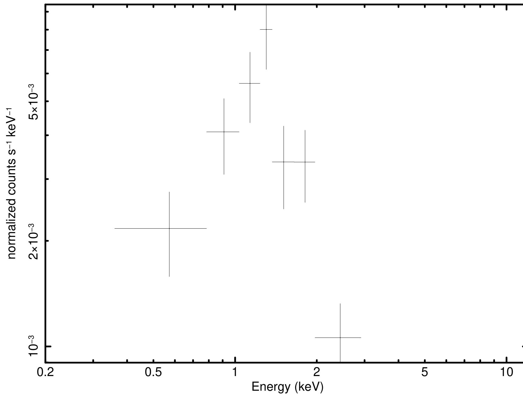
Source 6 minus background (P0921180301M2S002SRSPEC0006)
