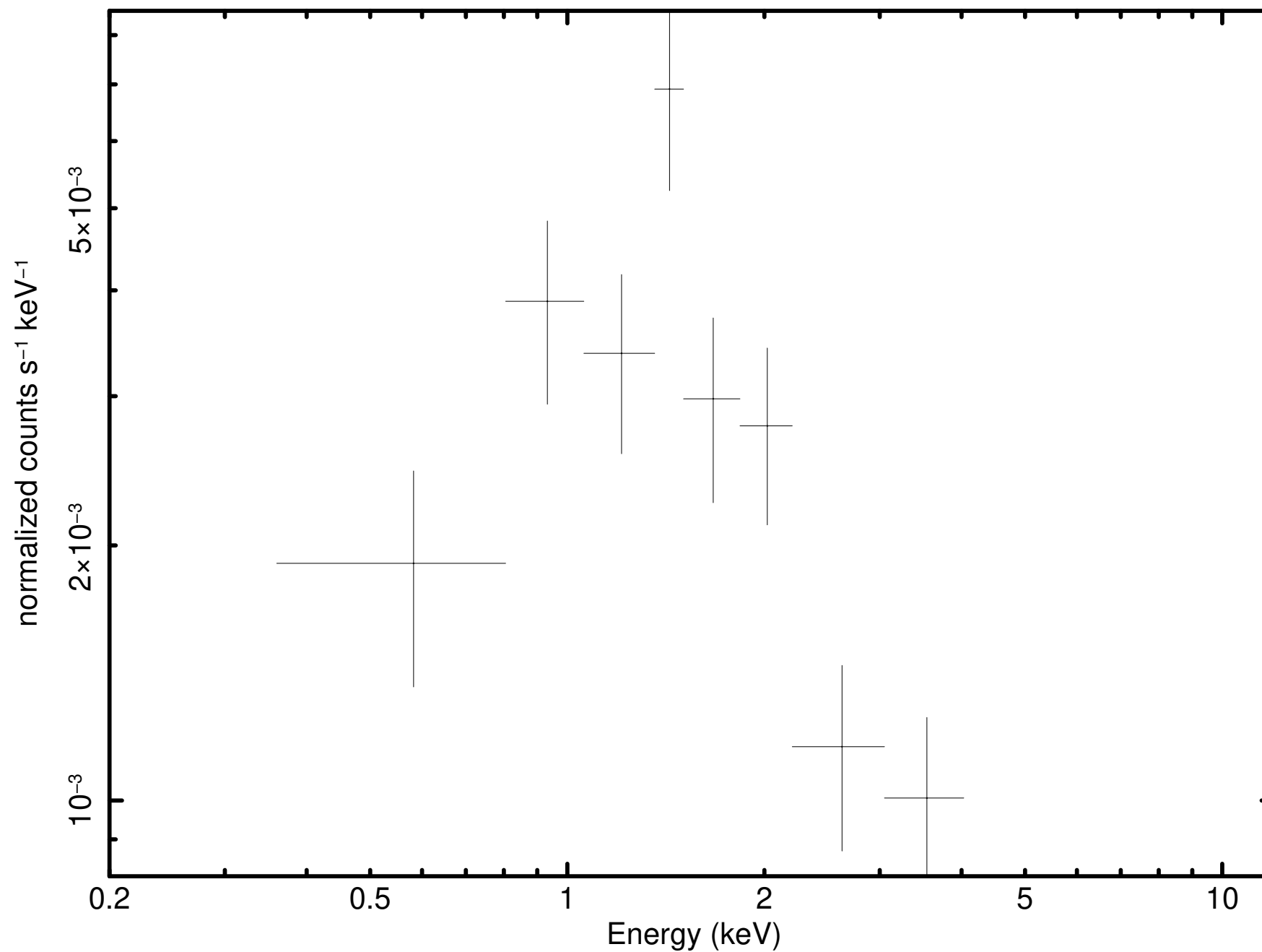
Source 7 minus background (P0921180301M2S002SRSPEC0007)
