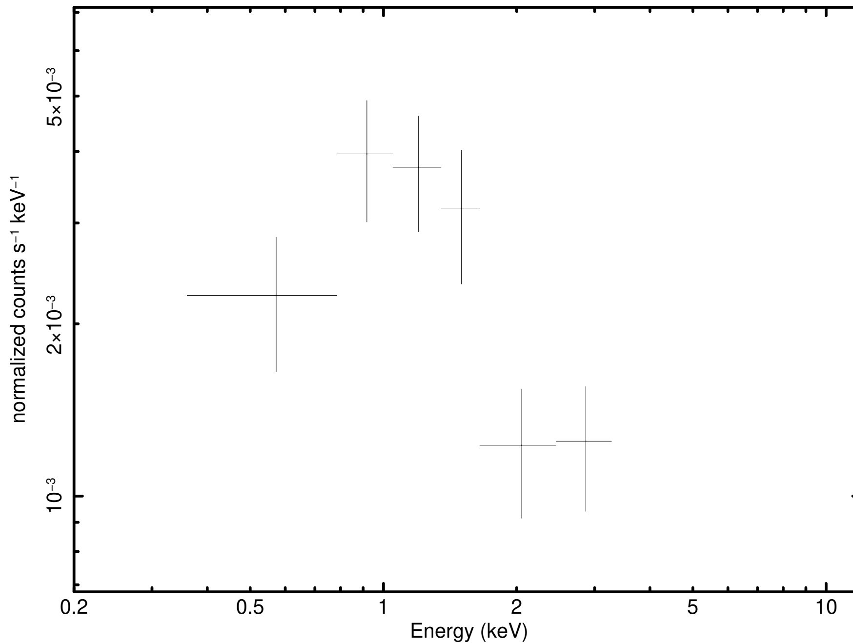
Source 10 minus background (P0921180301M2S002SRSPEC000A)
