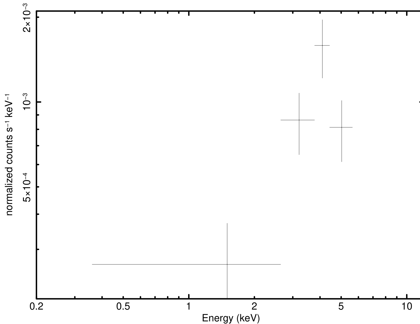
Source 16 minus background (P0921180301M2S002SRSPEC0010)
