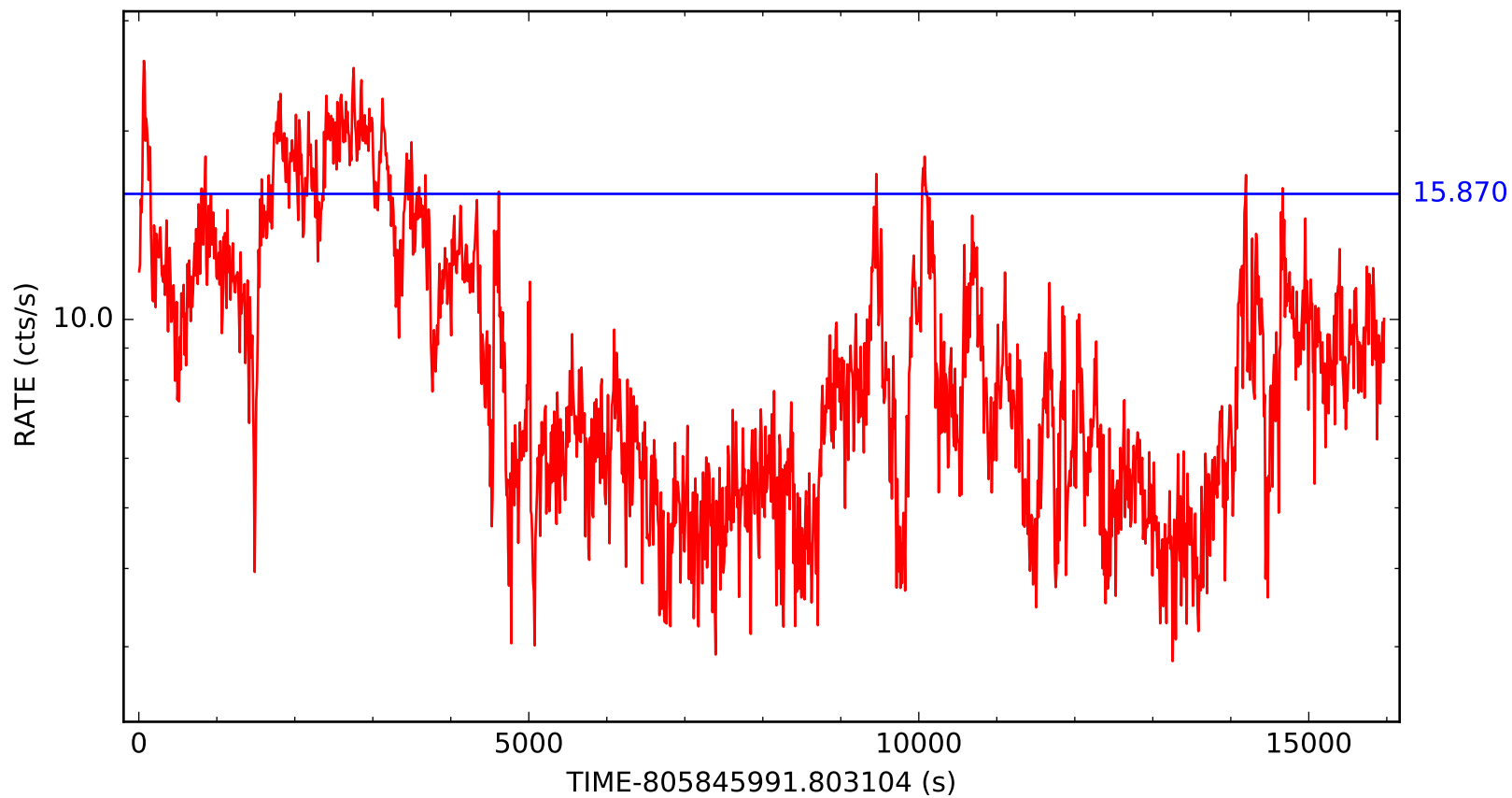
Plot of file P0921180301PNS003FBKTSR0000.FIT
