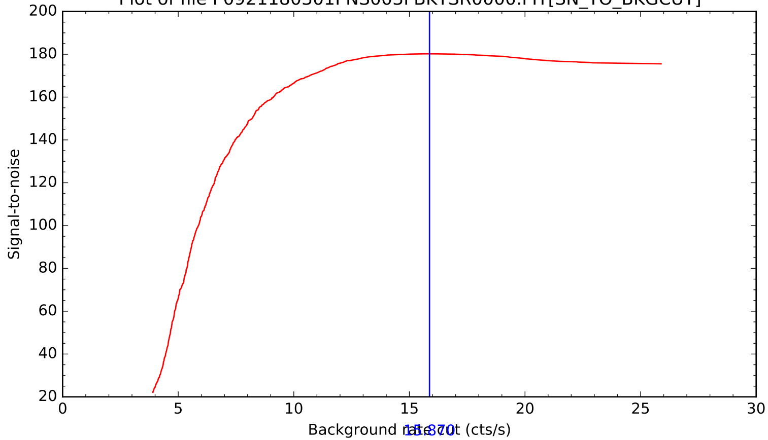
Plot of file P0921180301PNS003FBKTSR0000.FIT[SN_TO_BKGCUT]
