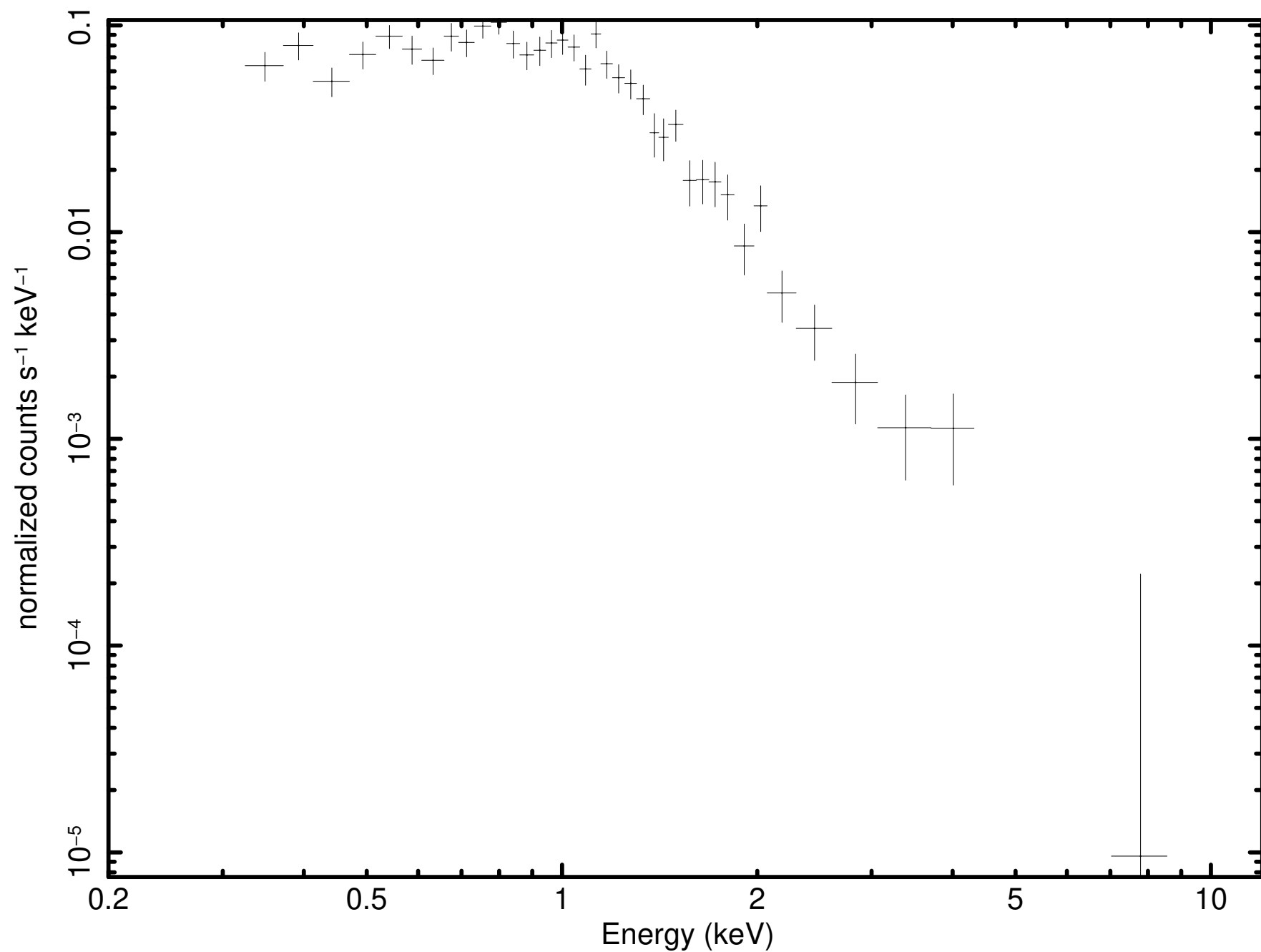
Source 1 minus background (P0921180301PNS003SRSPEC0001)
