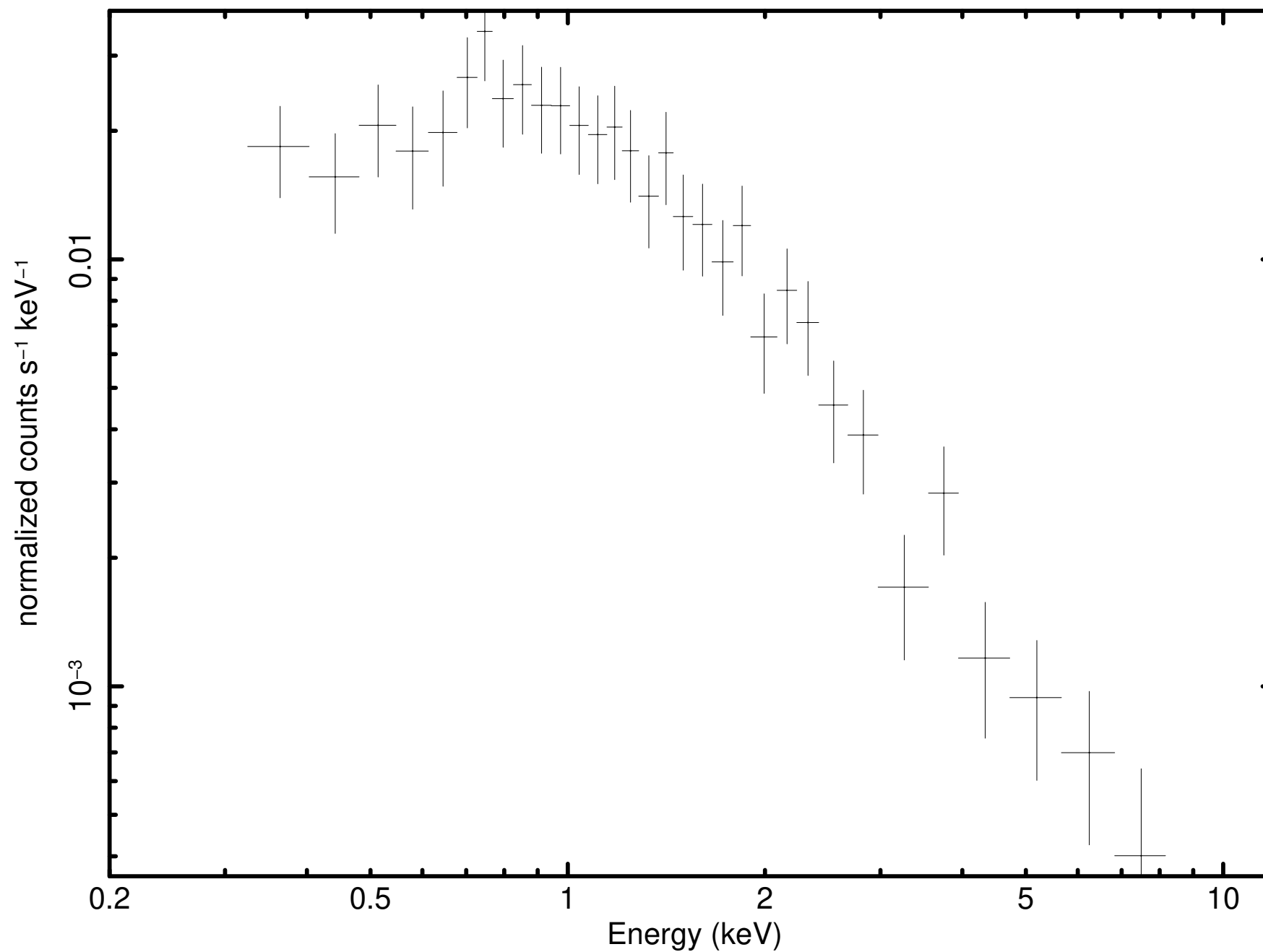
Source 2 minus background (P0921180301PNS003SRSPEC0002)
