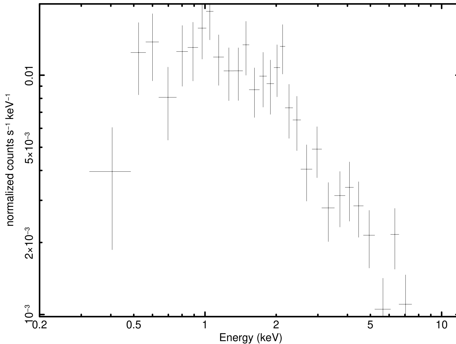
Source 3 minus background (P0921180301PNS003SRSPEC0003)
