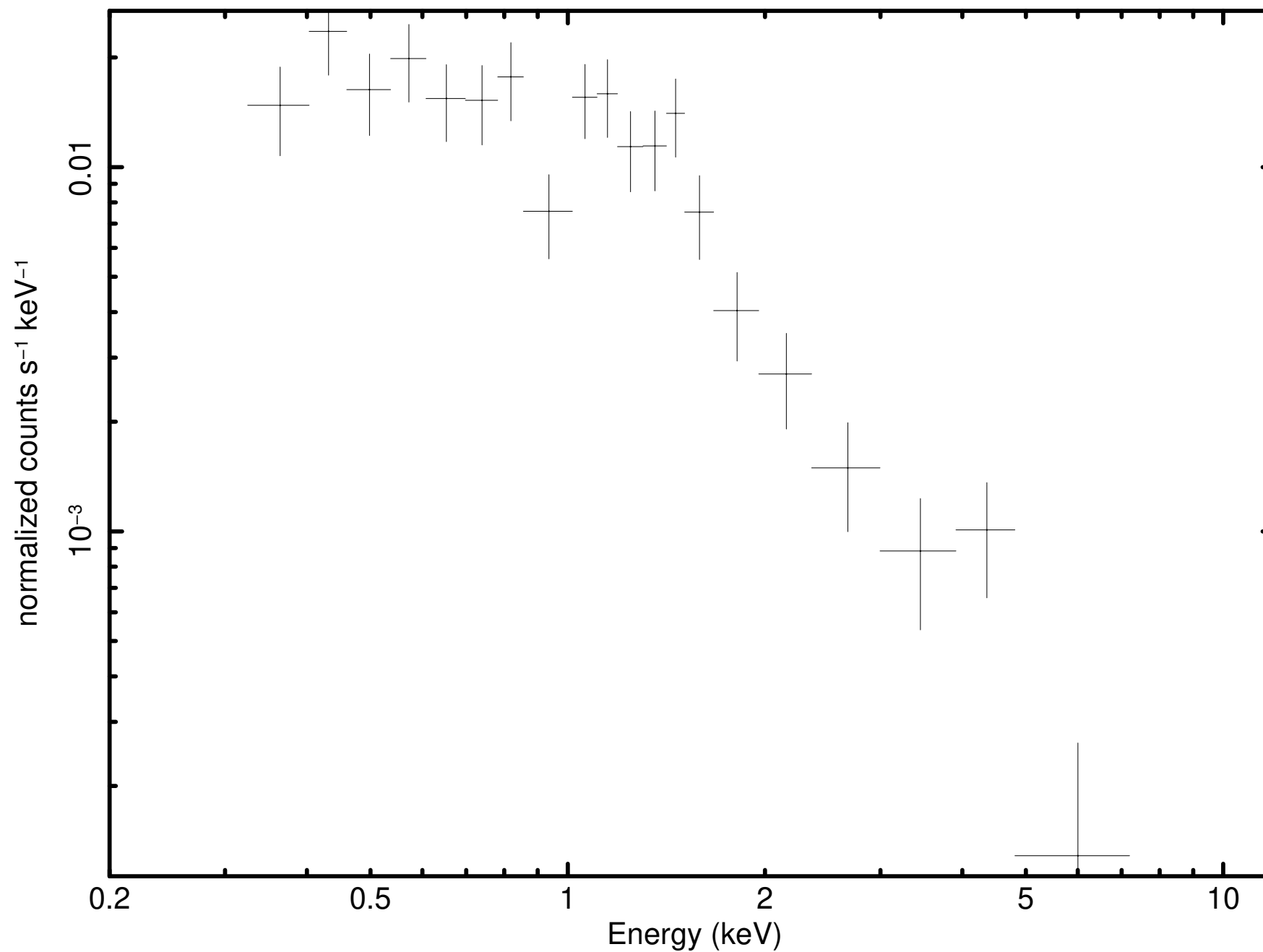
Source 5 minus background (P0921180301PNS003SRSPEC0005)
