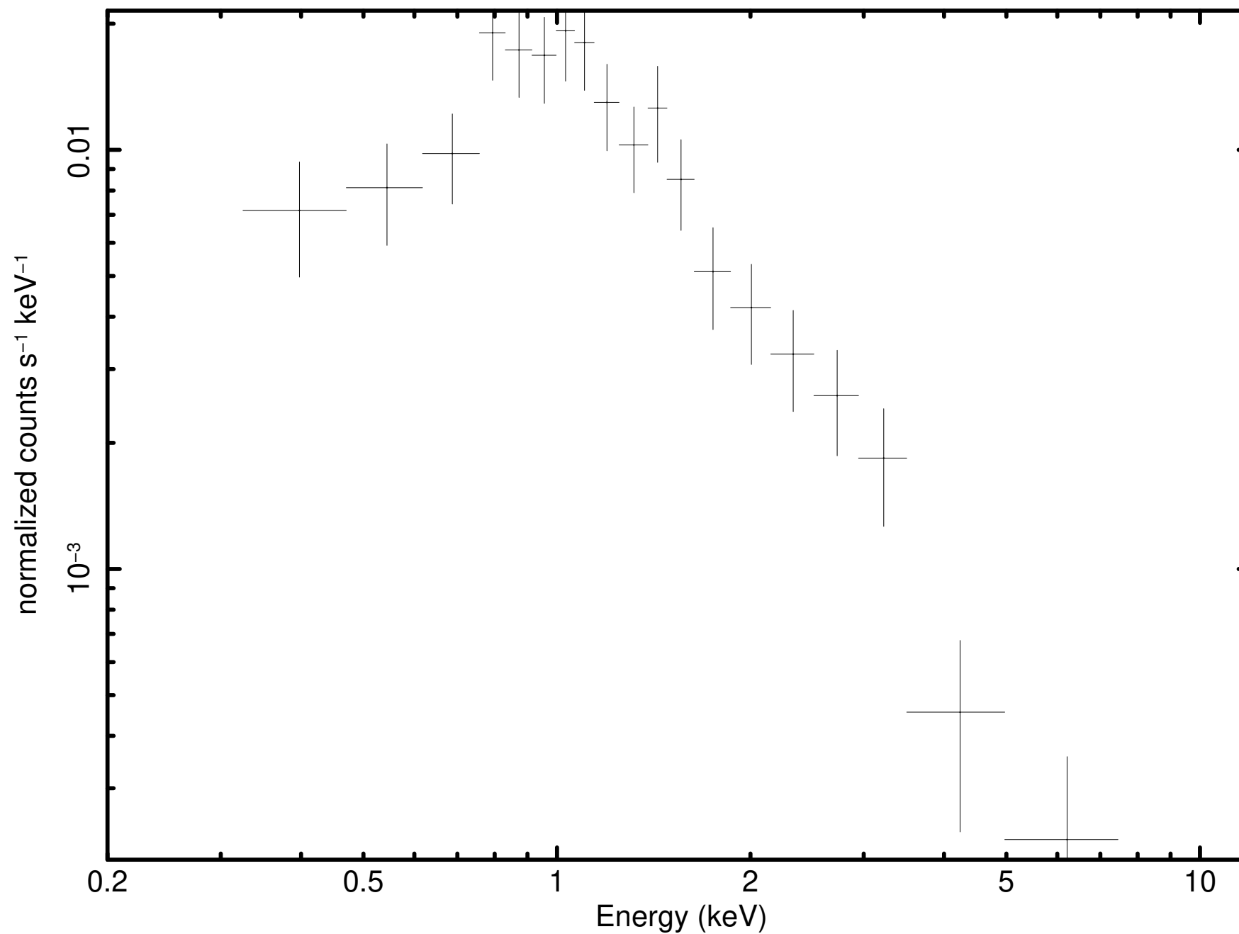
Source 6 minus background (P0921180301PNS003SRSPEC0006)
